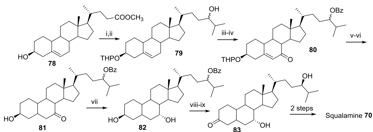
Figure 14. Synthesis of squalamine performed by Zhou et al. in 2019. Reagents and conditions: (i) DHP, PPTS, DCM; (ii) i-PrMgBr , \text{LiBH}_4 ; (iii) \text{BzCl} ; (iv) PDC, TBHP; (v) \text{H}_2 , Pd/C; (vi) HCl; (vii) L-selectride; (viii) \text{AgCO}_3/\text{Silica} ; (ix) KOH, MeOH
