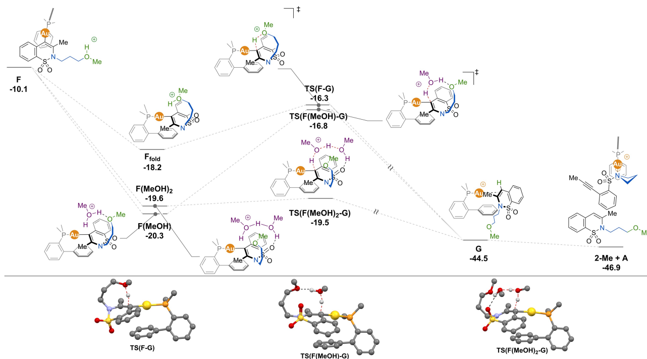
Scheme 3. Free energy reaction profile (kcal/mol) for the protodemetalation step using 1-Me as substrate computed at the B3LYP-D3(DCM)/LANL2TZ(f)/6-311 + +G**//LANL2DZ/6-31G** level of theory.
