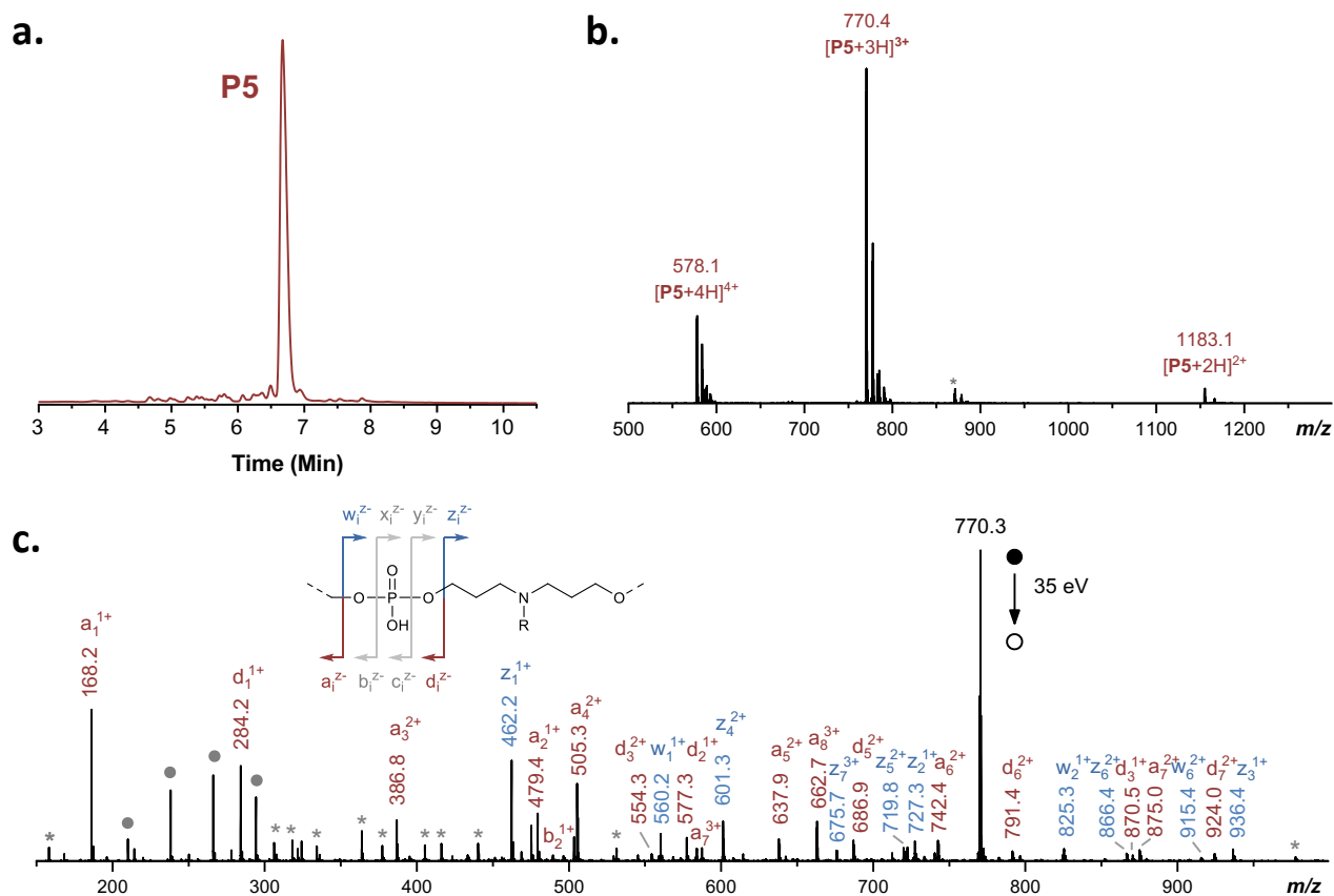
Figure 1. Characterization of copolymer P5 . (a) HPLC trace. (b) Positive mode ESI-MS. The grey asterisk indicates traces of DMT-protected polymer. All other unlabeled peaks are cation adducts. (c) MS/MS sequencing. This spectrum was obtained by collision-induced dissociation of [P5+3H]^{3+} . Grey asterisks denote internal fragments. The full grey circles indicate internal fragments corresponding to the four different coded subunits. The inset schematize the fragmentation pattern of a phosphate repeat unit. Light grey arrows indicate fragmentation series that are weakly detectable in these measurements.
