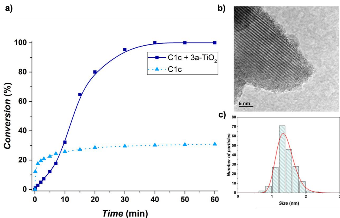
Figure 10. (a) Comparison of the catalytic activities for the C1c catalyst in the absence and in the presence of the 3a-TiO 2 material for the C-C coupling of p -bromoacetophenone and phenylboronic acid. Reaction conditions: 8 \times 10^{-4} mmol Pd, 0.8 mmol p -bromoacetophenone, 1 mmol phenylboronic acid, 1.2 mmol MeONa, 16 mL EtOH, 60°C. (b) TEM micrograph of the 3a-TiO 2 material with (c) its size histogram after the catalytic reaction.
