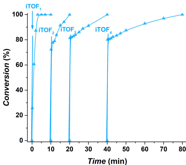
Figure 6. Recyclability (method A) of the mC1c -TiO 2 catalyst for the C-C coupling of p -bromoacetophenone and phenylboronic acid. Reaction conditions: 8 \times 10^{-4} mmol Pd, 0.8 mmol p -bromoacetophenone, 1 mmol phenylboronic acid, 1.2 mmol MeONa, 16 mL absolute EtOH, 60°C.
