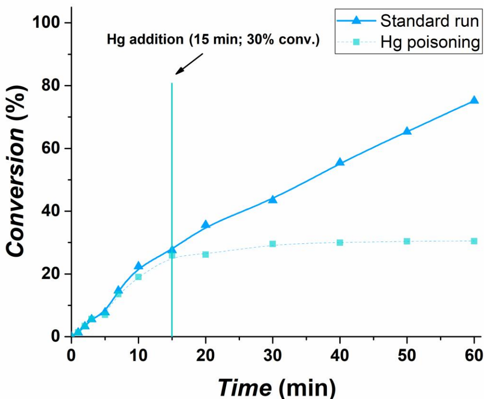
Figure 11. Comparison of the catalytic activities for mC1c -TiO 2 catalyst in the absence (standard run) and after the addition of Hg (Hg poisoning) for the coupling of p-bromoacetophenone and phenylboronic acid at 25°C.
