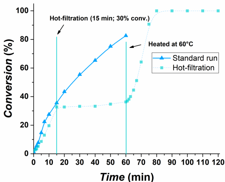
Figure 5. Activity of mC1c-TiO 2 catalyst after hot-filtration at ca. 30% conversion versus standard catalytic run.
