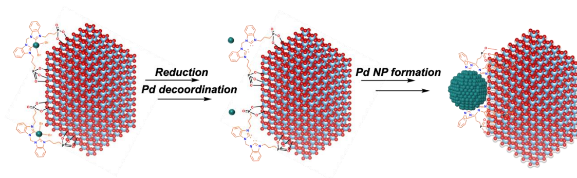
Scheme 3. Catalyst evolution of grafted Pd-bisNHC complexes at the surface of TiO 2 .
