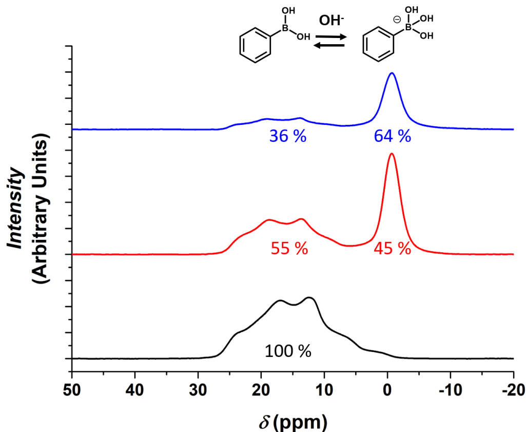
Figure 12. ^{11}\text{B} MAS NMR spectrum for the phenylboronic acid (black line), phenylboronic acid after 1 h reaction with 1.25 equivalents of MeONa in EtOH (red line) and phenylboronic acid after 1 h reaction with 1.25 equivalents of MeONa in the presence of 1 equivalent of \text{TiO}_2 in EtOH (blue line).
