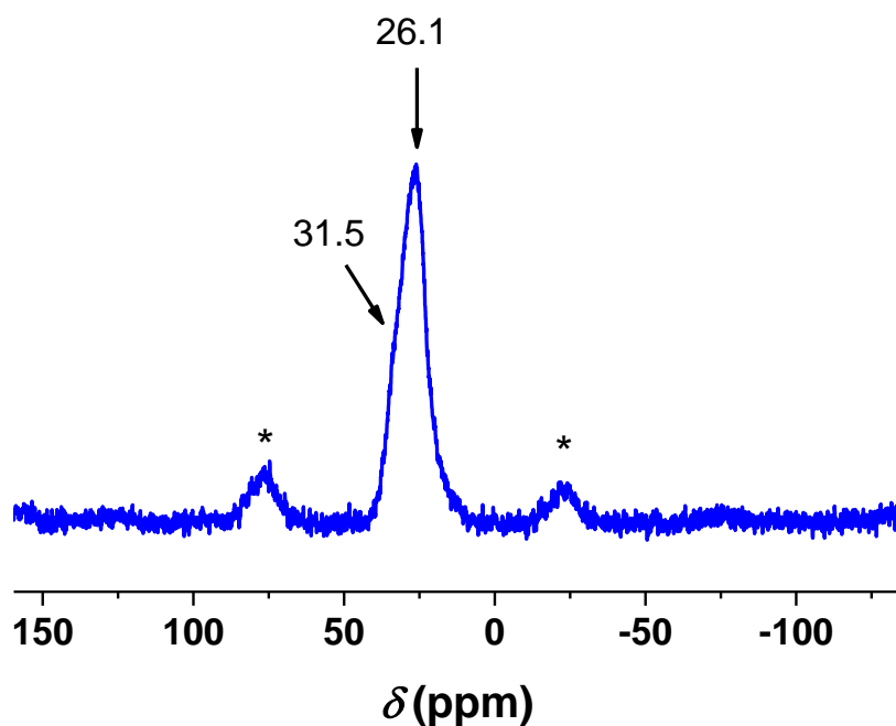
Figure 2. ^{31}\text{P} HPDEC NMR spectrum of mC1a-TiO 2 hybrid material. * Spinning bands.
