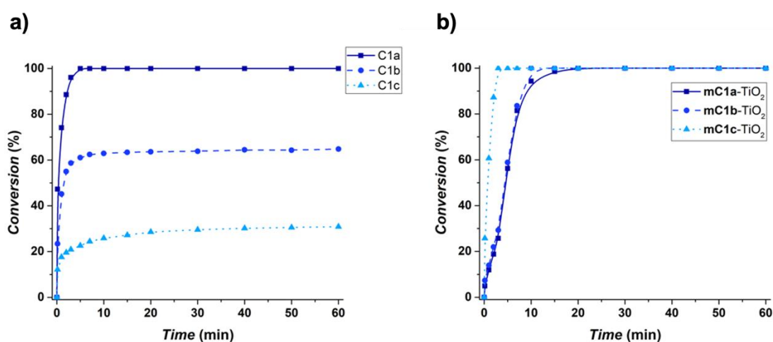
Figure 3. Conversion versus the time for the coupling reaction of p -bromoacetophenone with phenylboronic acid using (a) C1a-c and (b) mC1a-c-TiO 2 catalysts at 60°C.
