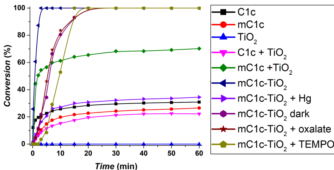
Figure 9. Catalytic performance for the coupling of p -bromoacetophenone and phenylboronic acid by using (a) C1c , black, squares, (b) mC1c , red, round, (c) \text{TiO}_2 , blue, triangle, (d) C1c + \text{TiO}_2 , pink, inversed triangle, (e) mC1c + \text{TiO}_2 , green, rhombus, (f) mC1c-TiO 2 , navy, left arrow, (g) mC1c-TiO 2 + Hg, violet, right arrow, (h) mC1c-TiO 2 in the dark, purple, hexagon, (i) mC1c-TiO 2 + sodium oxalate, brown, stars, (j) mC1c-TiO 2 + TEMPO, olive, pentagon.
