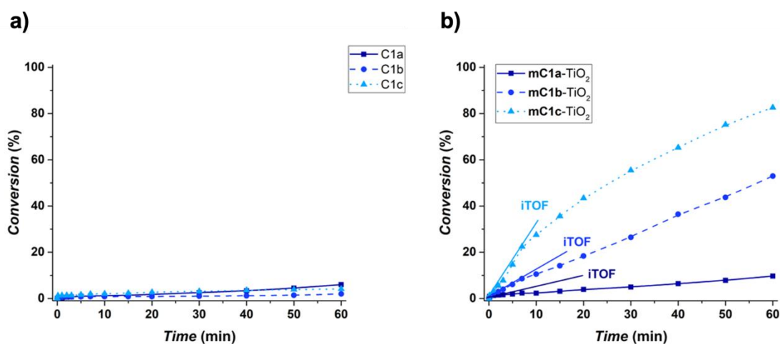
Figure 4. Conversion versus the time for the coupling reaction of p -bromoacetophenone with phenylboronic acid using (a) C1a-c and (b) mC1a-c-TiO 2 catalysts at 25°C.
