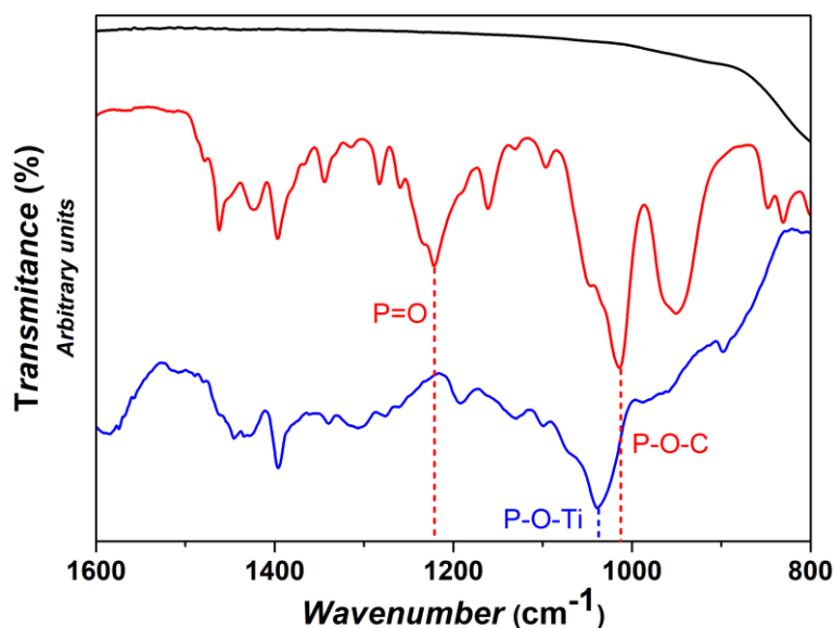
Figure 1. Overlay of ATR-IR spectra of \text{TiO}_2 (black), mC1a complex (red) and mC1a-TiO 2 hybrid material (blue). The transmittance of each sample has been shifted along the y-axis for comparison purposes.
