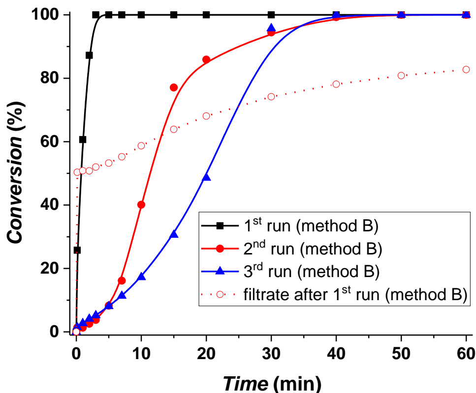
Figure 7. Recyclability (method B) of the mC1c -TiO 2 catalyst for the C-C coupling of p -bromoacetophenone and phenylboronic acid. Reaction conditions: 8 \times 10^{-4} mmol Pd, 0.8 mmol p -bromoacetophenone, 1 mmol phenylboronic acid, 1.2 mmol MeONa, 16 mL absolute EtOH, 60°C.
