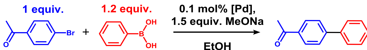
Scheme 2. Suzuki-Miyaura reaction studied in this work.
