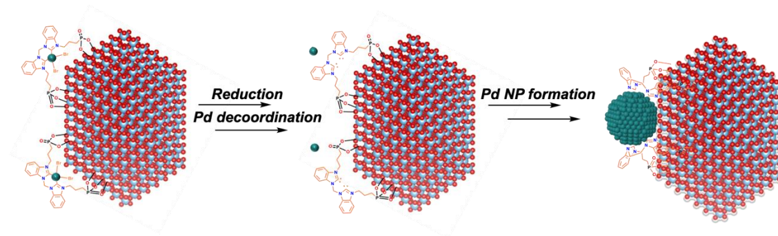
Scheme 3. Catalyst evolution of grafted Pd-bisNHC complexes at the surface of TiO 2 .
