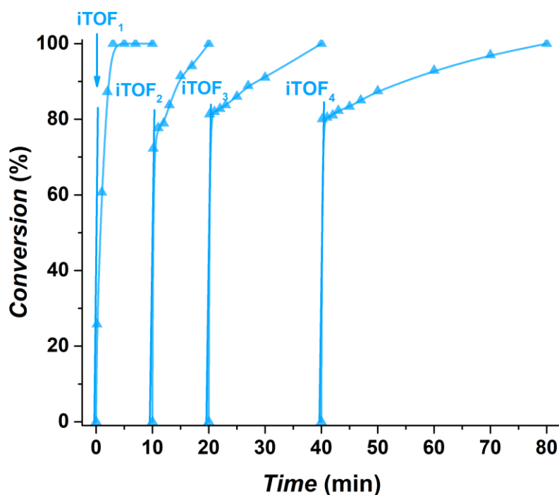
Figure 6. Recyclability (method A) of the mC1c-TiO 2 catalyst for the C-C coupling of p -bromoacetophenone and phenylboronic acid. Reaction conditions: 8 \times 10^{-4} mmol Pd, 0.8 mmol p -bromoacetophenone, 1 mmol phenylboronic acid, 1.2 mmol MeONa, 16 mL absolute EtOH, 60°C.
