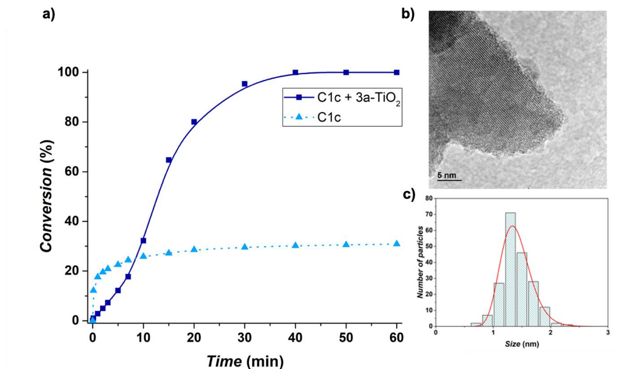
Figure 10. (a) Comparison of the catalytic activities for the C1c catalyst in the absence and in the presence of the 3a-TiO 2 material for the C-C coupling of p -bromoacetophenone and phenylboronic acid. Reaction conditions: 8 \times 10^{-4} mmol Pd, 0.8 mmol p -bromoacetophenone, 1 mmol phenylboronic acid, 1.2 mmol MeONa, 16 mL EtOH, 60°C. (b) TEM micrograph of the 3a-TiO 2 material with (c) its size histogram after the catalytic reaction.
