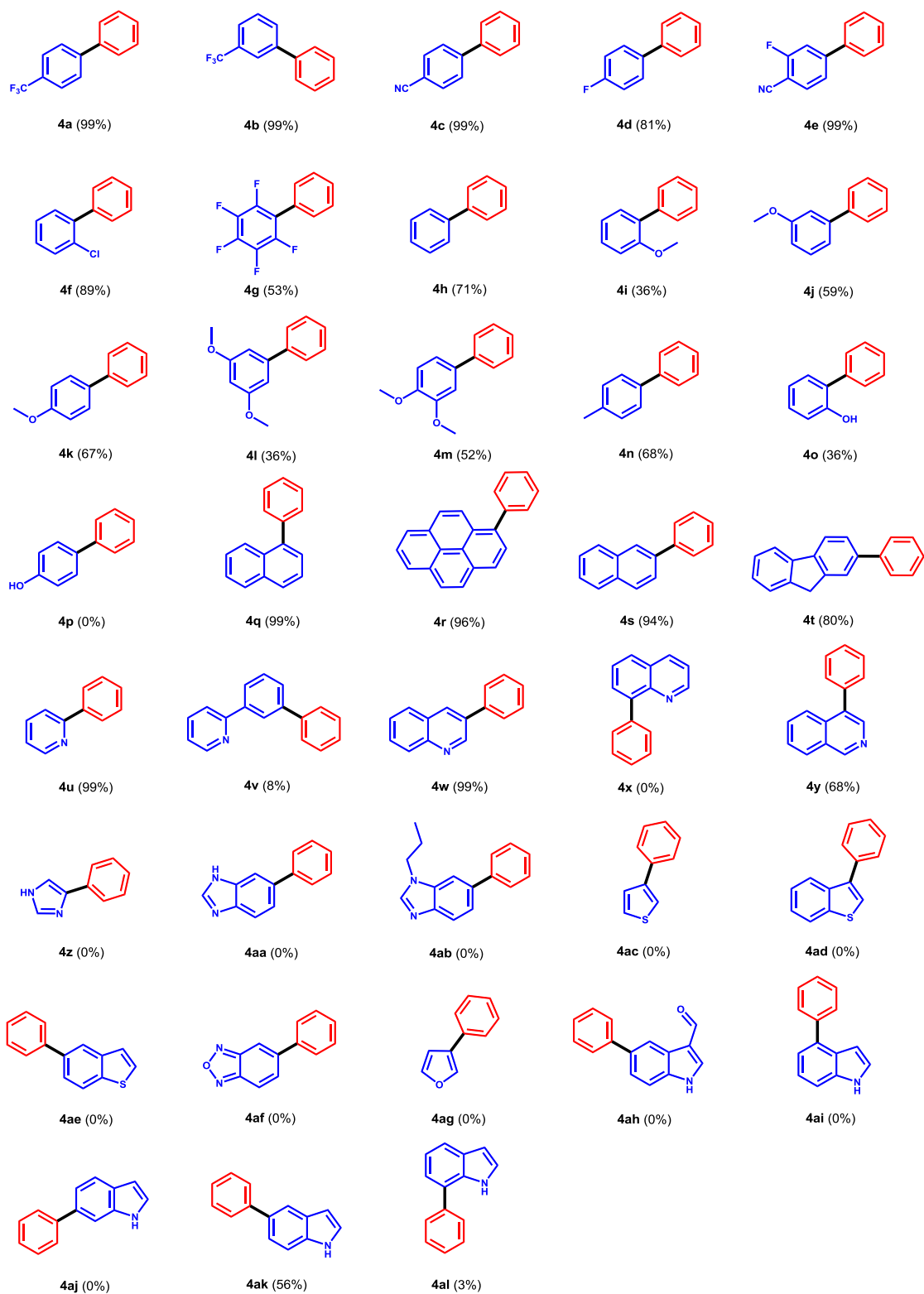
Figure 13. Reaction scope for the coupling of aryl bromides with phenylboronic acid in the presence of the mC1c-TiO 2 catalyst.
