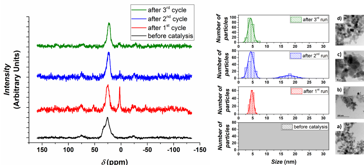
Figure 8. Evolution of the 31 P HPDEC NMR for the mC1c -TiO 2 catalyst upon recycling and TEM images with their Pd NPs size histograms for each run (method B).
