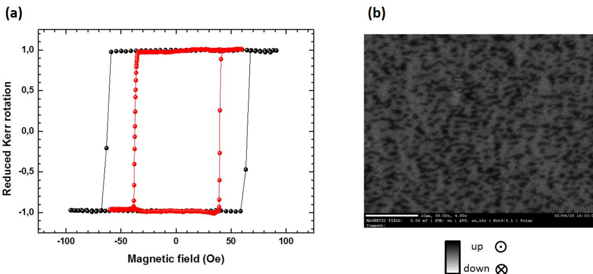
Figure S1. (a) Hysteresis loops performed with a polar magneto-optical Kerr effect (MOKE) microscope on Si//Ta(5)/Ir(5)/Fe(0.3)/Gd 26.1 Fe 65.5 Co 8.3 (8)/Pt(5) before (Black) and after milling (red). (b) Image taken with a MOKE microscope at RT after nucleation using an IP magnetic field. Scale bar: 10 μm.
