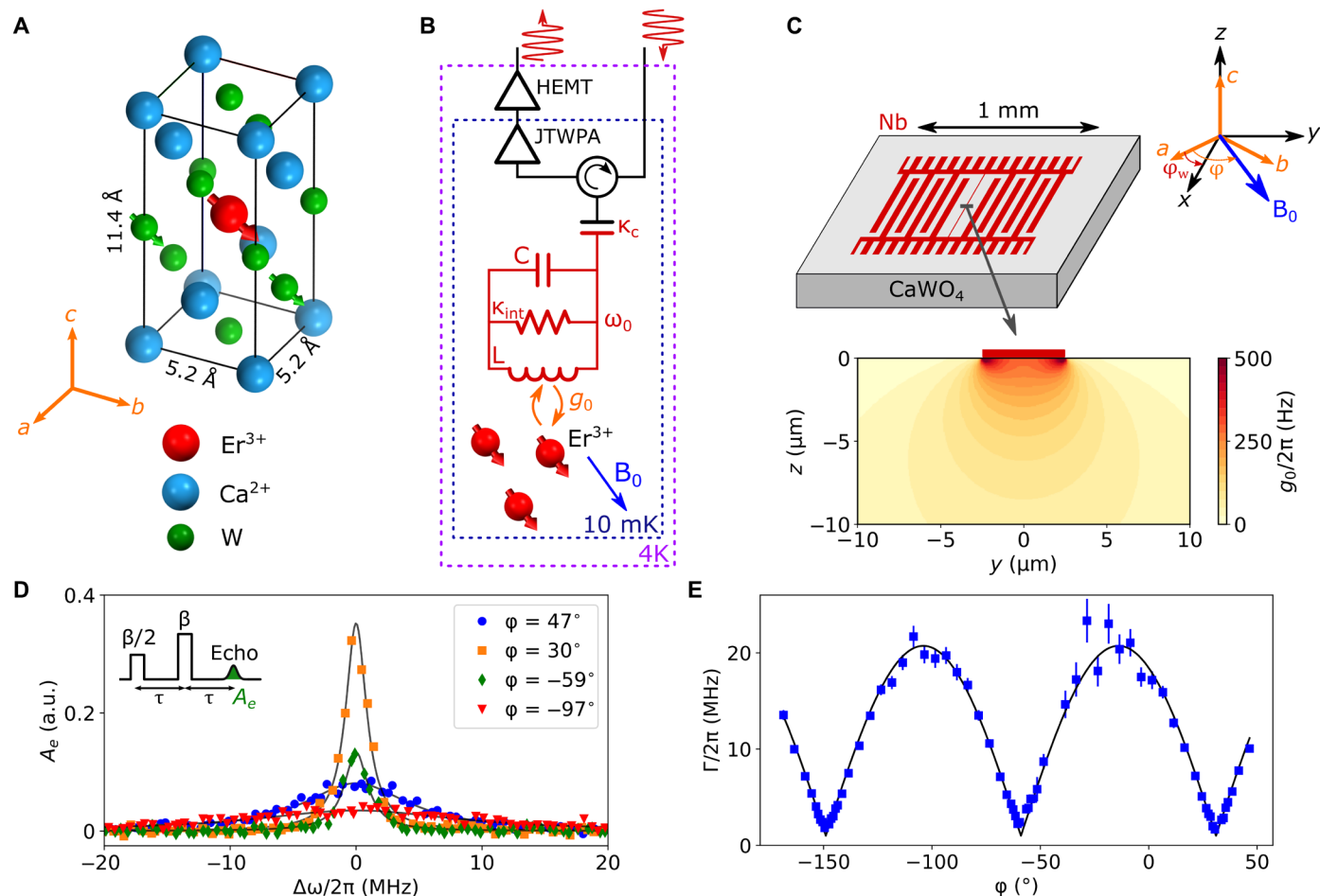
Fig. 1. Schematics of the experiment and erbium spins spectroscopy. (A) Unit cell of CaWO 4 with a central Er 3+ dopant. Oxygen atoms are removed for clarity. A fraction 0.14 of tungsten atoms has a nuclear spin. (B) Experimental EPR setup. The erbium spins, subjected to a magnetic field B_0 , are coupled with strength g_0 to an LC resonator. The latter has an internal loss rate \kappa_{\text{int}} and is coupled to a measurement line with rate \kappa_c . Microwave pulses are sent to the device, and the reflected signal containing the spin echo is routed toward a JTWPA (Josephson traveling-wave parametric amplifier), followed by a HEMT (high-electron-mobility transistor) at 4 K and by further amplification and demodulation at room temperature. (C) Sketch of one of the three 50-nm-thick niobium LC resonators fabricated on top of the CaWO 4 sample, in the ab plane. The dc magnetic field B_0 is applied in the ab plane at an angle \varphi with respect to the a axis, the resonator inductor making an angle \varphi_w with this axis. The cross section shows the coupling g_0 between the resonator and erbium spins around the 5- \mu\text{m} -wide inductance wire when B_0 is applied along its direction ( x axis). (D) Spin echo integral A_e as a function of B_0 , around 67.2 mT, converted into a frequency detuning \Delta\omega . Full symbols are measurements for various values of \varphi , whereas solid lines are Lorentzian fits to the data which are plotted in arbitrary units (a.u.). (E) Full width at half maximum linewidth \Gamma/2\pi as a function of \varphi . The solid line is a fit following the model of (26, 27), yielding a typical magnitude of inhomogeneous electric fields along the c axis of 32 kV/cm.
