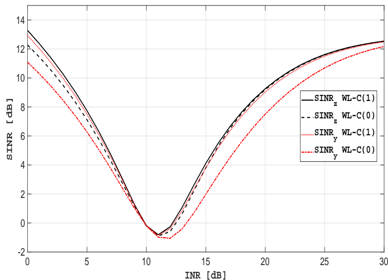
Fig. 2. SINR and \text{SINR}_z at the output of the WL-C(1) and WL-C(0) MMSE receivers as a function of the INR for N = 1 , BPSK SOI and CCI with \tau_j = 0 , \phi = 0 and \text{SNR} = 10\text{dB} .
