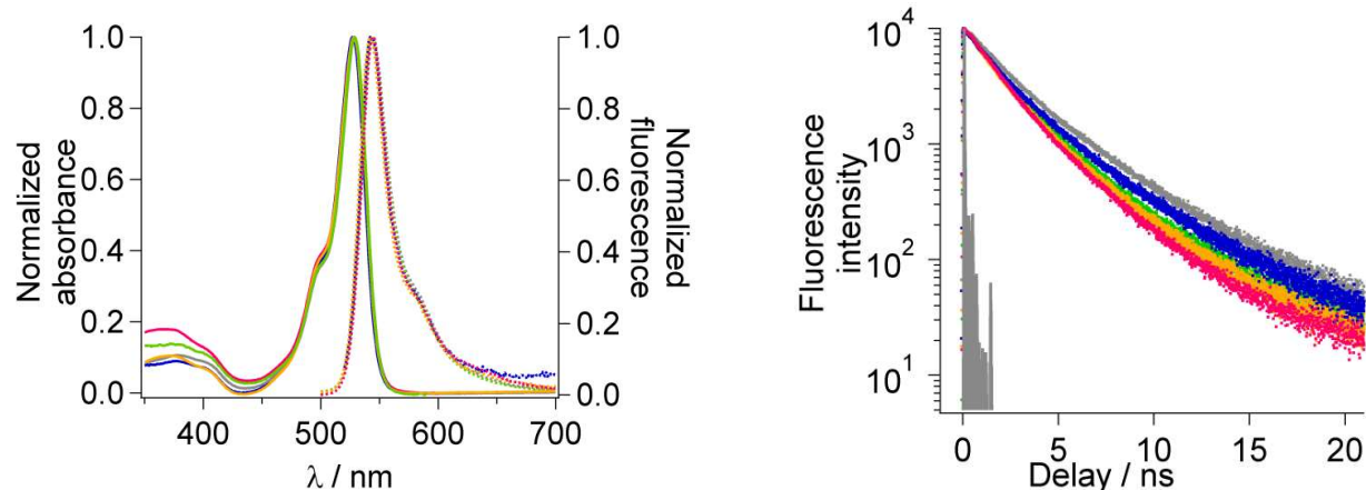
Figure 8. Spectra of nanoparticles with different BODIPY monomers ( \pi PhMA (—), \pi PhA (—), \pi EtMA (—), \pi EtA (—), \pi S (—) recorded in water. Left: absorption (full lines) and emission (dotted lines, \lambda_{\text{exc}} = 495 nm) spectra. Right: fluorescence decays (grey line is the instrument response function, \lambda_{\text{exc}} = 495 nm, \lambda_{\text{F}} = 543 nm).
