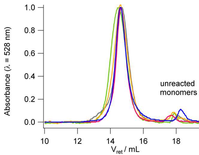
Figure 6. Size exclusion chromatograms (UV-vis. detection, \lambda = 528 nm) in THF for polymer chains of nanoparticles with different BODIPY monomers ( \pi PhMA 1 (—), \pi PhA 2 (—), \pi EtMA 3 (—), \pi EtA 4 (—), \pi S 5 (—)).
