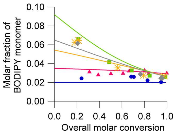
Figure 7. Evolution of the average molar fraction of BODIPY monomer in the copolymer with the overall molar monomer conversion (symbols: experimental values, — calculated with the reactivity ratios; initial molar fraction of BODIPY monomer = 2.6 mol%). Monomers \pi PhMA 1 ( \blacksquare —, r_S = 0.25 , r_{\text{PhMA}} = 0.50 18 ), \pi PhA 2 ( \blacklozenge —, r_S = 0.38 determined by the Kelen-Tüdös method, r_{\text{PhA}} estimated at 0.50) 31 , \pi EtMA 3 ( \blackast —, r_S = 0.46 , r_{\text{EtMA}} = 0.38 32 ), \pi EtA 4 ( \blacktriangle —, r_S = 0.8 , r_{\text{EtA}} = 0.2 33 ), \pi S 5 ( \bullet —, r_S = 1 , r_S = 1 ).
