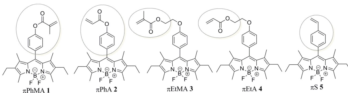
Figure 1. Molecular structure of the BODIPY monomers possessing different polymerizable functions.
