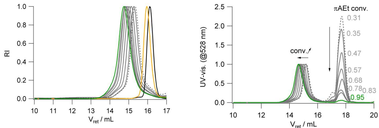
Figure 5. Monitoring of the synthesis of nanoparticles 4 (with \pi EtA) by size exclusion chromatography in THF. Left: RI detection. Right: UV-vis. detection at the maximal absorption of the monomer \pi EtA 4 ( \lambda = 528 \text{ nm} ). (macro-RAFT agents : — PEO-C 12 , — PEO- b -PAA-C 12 , PEO- b -PAA- b -P(S-co- \pi )-C 12 : ... end of bulk polymerization, — during miniemulsion polymerization, — end of miniemulsion polymerization.
