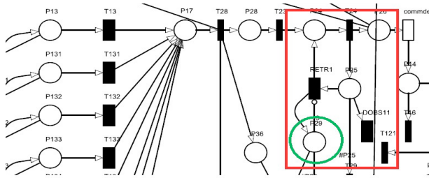
Fig. 12. part of SPN model: platoon with two VCTS unit
