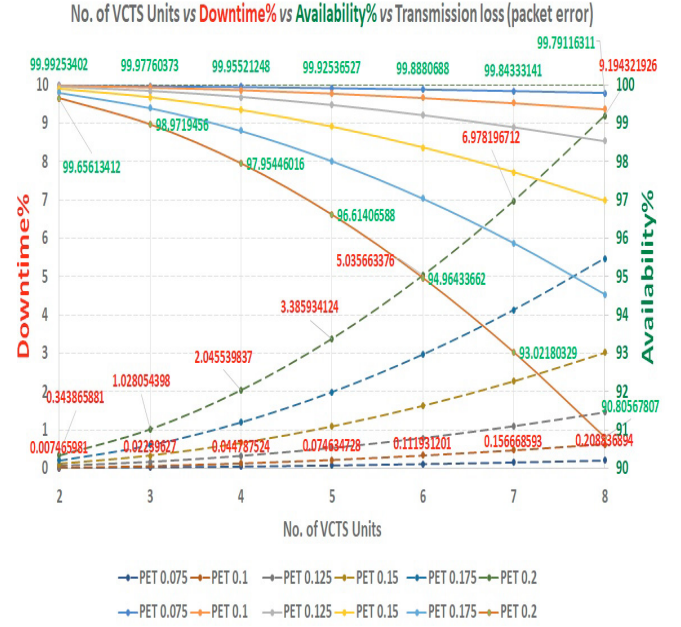
Fig. 7. Impact of platoon size and packet error on dependability attribute
