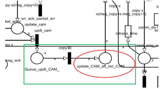
Fig. 11. Queuing at VCTS while processing of periodic CAM messages
