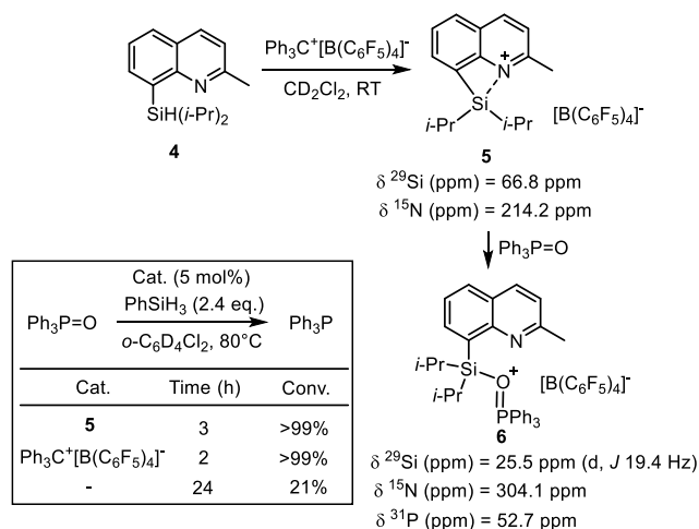
Scheme 1. Silyl cation complex with \text{Ph}_3\text{P}=\text{O} . Silylium mediated reduction of \text{Ph}_3\text{P}=\text{O} .
