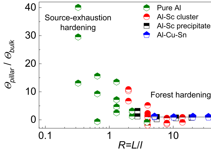
Figure 7. The hardening transition in FCC (Al and Al alloys) micropillars. The normalized strain-hardening rate \Theta_{pillar}/\Theta_{bulk} is shown a function of the dimensionless ratio R . A transition from forest hardening to source-exhaustion hardening is observed around R \approx 5 , whatever the material, in excellent agreement with the mild-to wild transition in Figure 5(b). Adapted with permission from [64].
