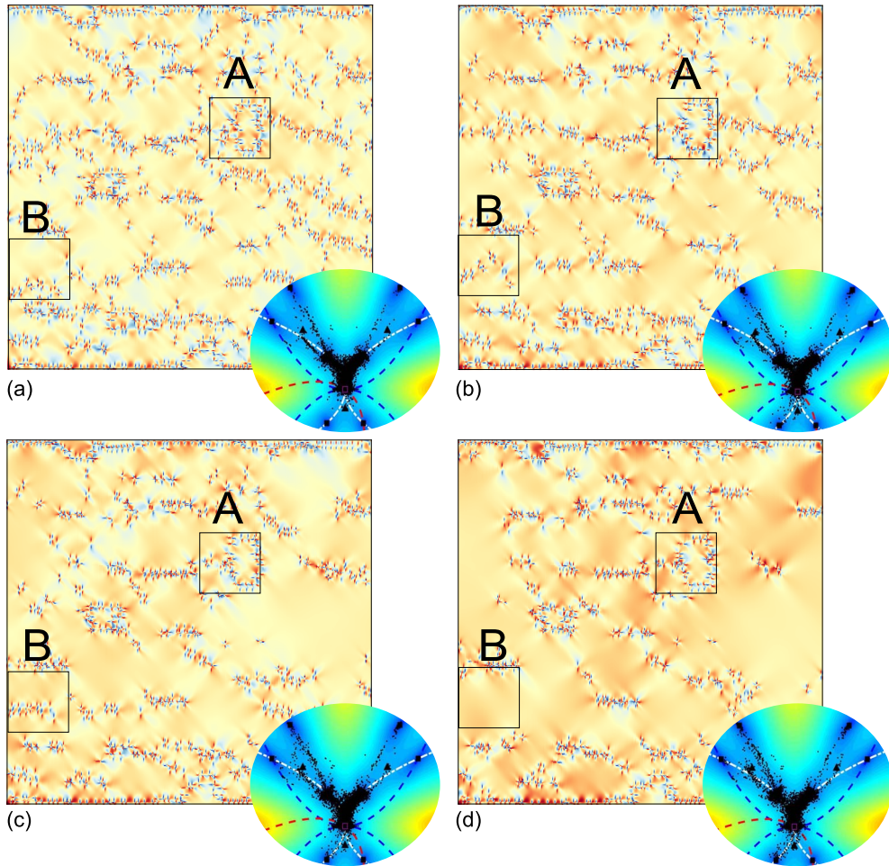
Figure 23. Evolution of the shear component of Cauchy stress in physical space after the catastrophic system-size avalanche. The snapshots correspond to the selected points in Figure 22 marked by numbers 1, 2, 3, 4. The corresponding distributions in the configurational space are shown in the insets. Here N = 500 and \phi = 0 .
