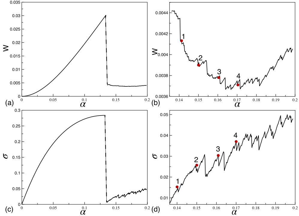
Figure 22. Macroscopic mechanical response of square crystal upon loading beyond the catastrophic system-size avalanche. Here N = 500 and \phi = 0 .
