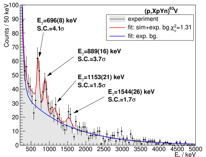
Figure 1. Doppler corrected \gamma -ray spectrum for ^{63}\text{V} using vertex reconstruction (requiring at least one proton in the TPC) and adback procedure including all reaction channels. The data with error bars and shaded area represent the experimental spectrum, the red line is the simulation plus a free-parameter double-exponential background, and the latter function (exponential background) is also plotted separately as a blue line. S.C. stands for the statistical confidence of the peaks.
