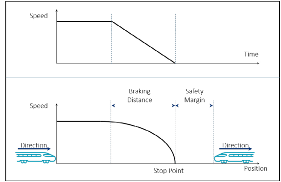
Fig. 4. Braking Distance
