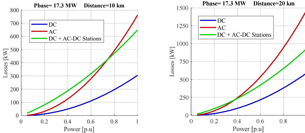
Fig. 3 – Power losses in function of the power for the point-to-point transmission at fixed distances for the voltage level of 10 kVac / ±10 kVdc.
