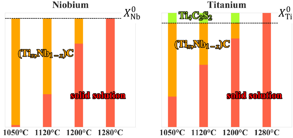
Fig. 4. Distribution of Nb and Ti for the investigated heat treated states, assuming that solute elements in (Ti,Nb)N remain trapped. Between 1280 and 1200°C, Nb evolution is only related to the formation of (Ti x Nb 1-x )C whereas Ti is affected by the formation of (Ti x Nb 1-x )C and Ti 4 C 2 S 2 .
