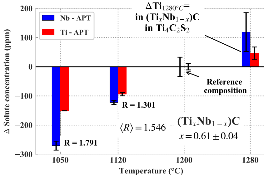
Fig. 5. Determination of x based on the respective evolution of Ti and Nb in solid solution below 1200°C. The total amount of Ti and Nb available for (Ti x Nb 1-x )C is deduced from the analysis.
