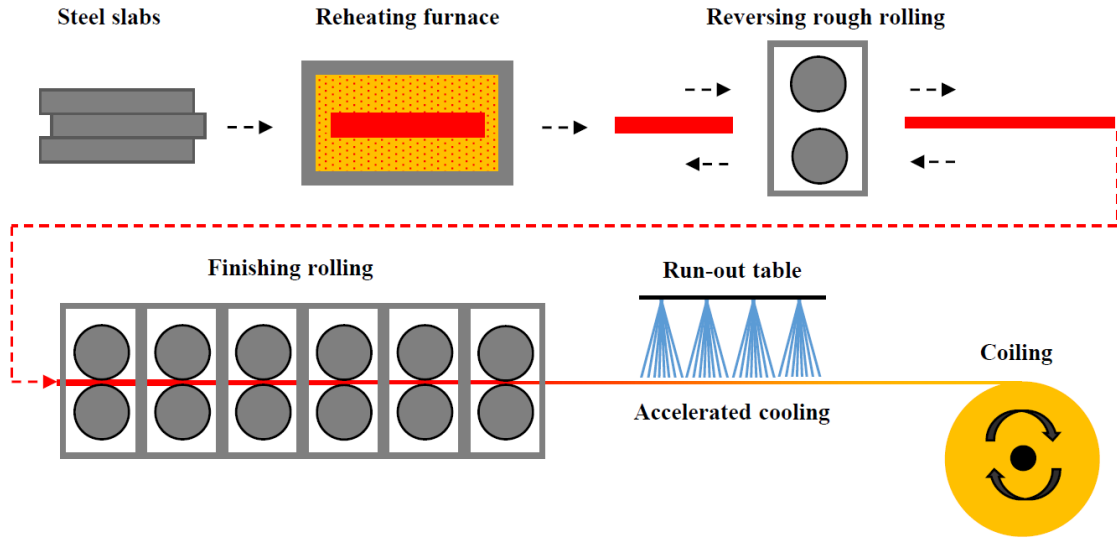
Figure 1. Schematic representation of the elaboration process of a bainitic steel sheet.
