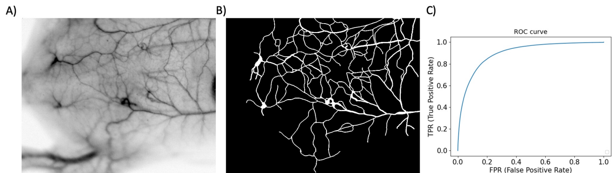
FIG. 1. a) Original SWIR image used for training; b) annotation of ground truth; c) Resulting receiver operating characteristic (ROC) curve of the performance of the training on SWIR images. Area under the curve: 0.90; Area under precision-recall curve: 0.57, Jaccard similarity score: 0.89
