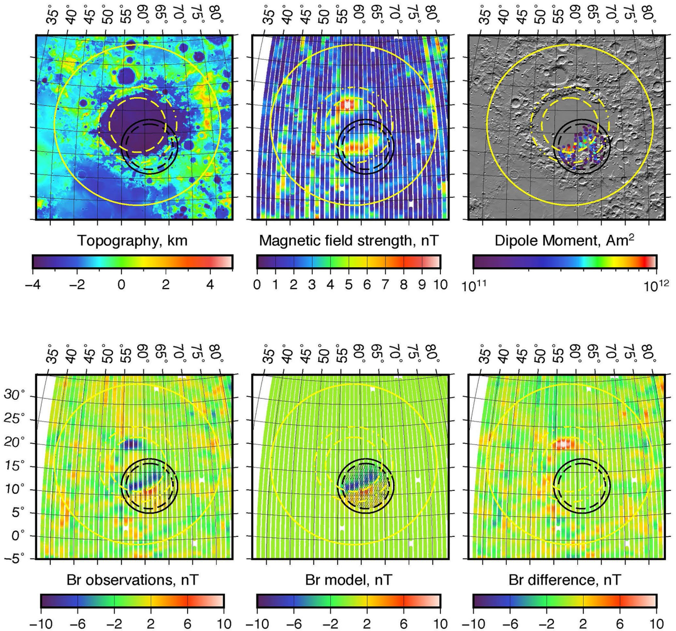
Figure 5. As in Figure 4 but for the southern Crisium anomaly.
