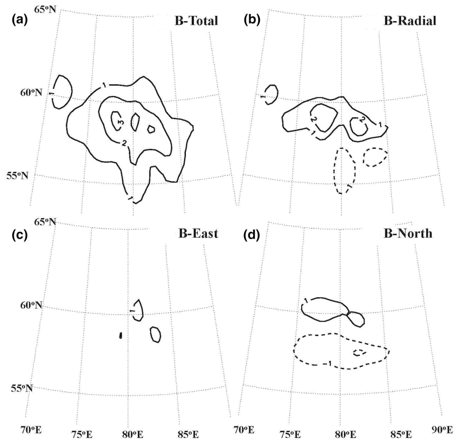
Figure 7. As in Figure 3 but for the Humboldtianum anomaly.
