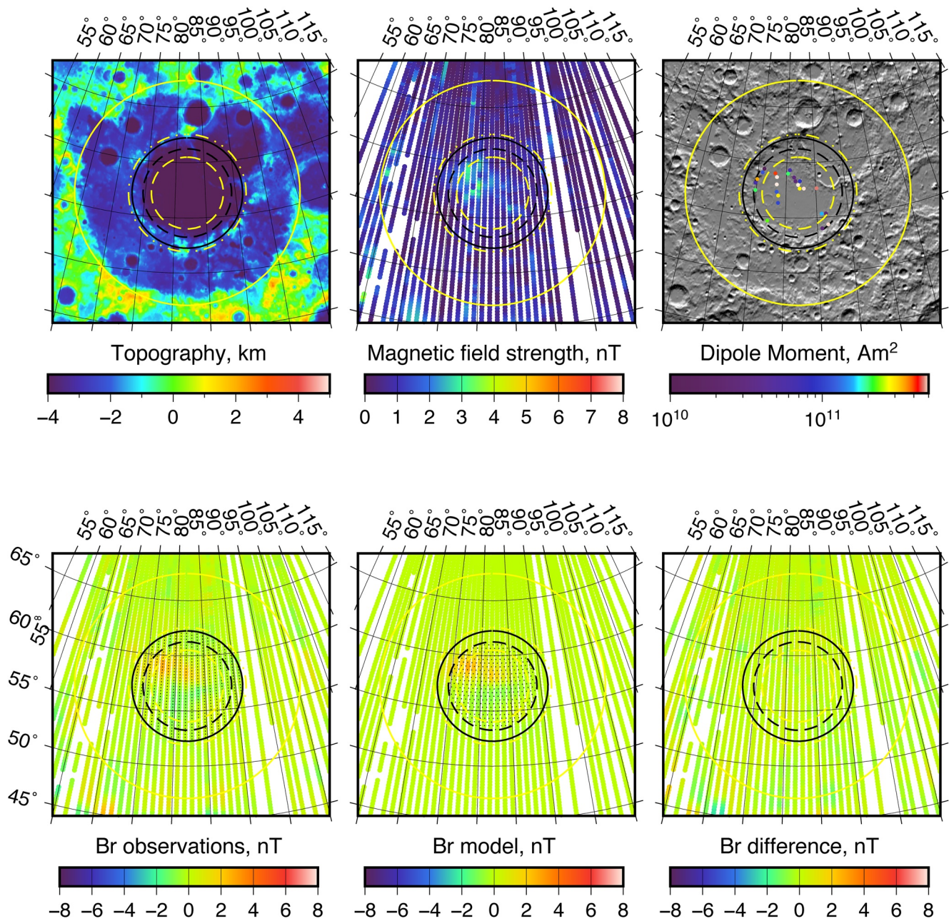
Figure 8. As in Figures 5 and 6 but for the Humboldtianum anomaly. Selected LP orbit segments from April 1999 are used (see the text).
