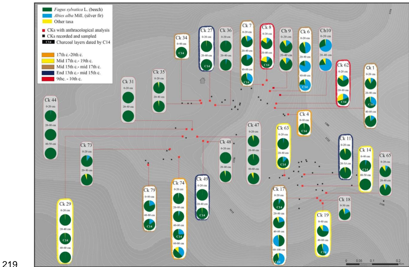
219 220 Fig. 5. Results of charcoal analysis by charcoal kilns (CKs) and by charcoal layers (CLs) in the Bernadouze 221 forest.
