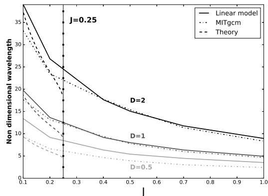
FIG. 3. Lee waves wavelength function of stability calculated from Eq. (19) (dashed), linear model (solid) and MITgcm model (dash-dotted). Each grey scale stand for a different value of D .
