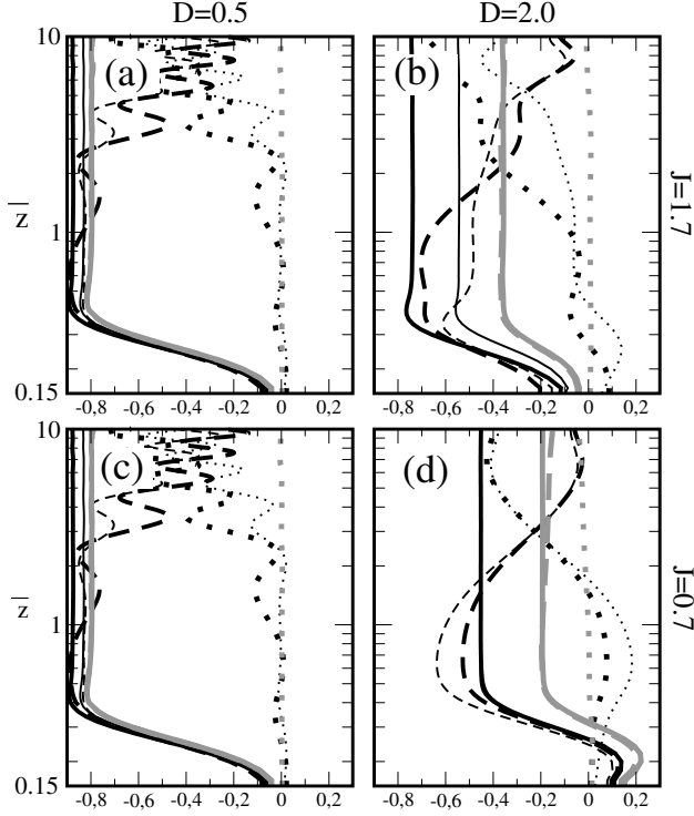
FIG. 8. Vertical profile of P^z (dashed), P^x (dot) and the sum ( P^{\text{out}} , solid) for different downstream position: \bar{X} = 3 (thick black); \bar{X} = 5 (thin black); and \bar{X} = 25 (thick grey).
