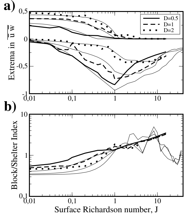
Fig. 6. Diagnostics from the MITgcm runs for S = 0.15 and for different values of the boundary layer depths D . In all panels, the corresponding results from the theory are in thin solid. a) Normalized extrema in momentum flux. b) Downslope sheltering versus upstream blocking index defined as the ratio between the max downslope wind amplitude and the max upslope wind amplitude (Eq. 28 from Part II):
