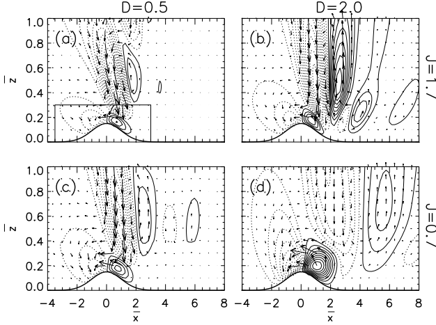
Fig. 7. Contours of vertical action component ( F^z ), negative values are dashed, along with total action vector for S = 0.15 . For illustration in a) are the limit of a characteristic box used to calculate the emitted PM fluxes.
