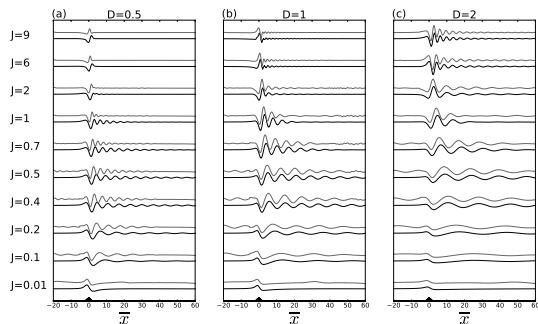
FIG. 2. Horizontal profiles of vertical velocity at \bar{z} = D for S = 0.15 . Each panel corresponds to a value of D and each line to a value of J . Profiles from the MITgcm model are represented in grey.
