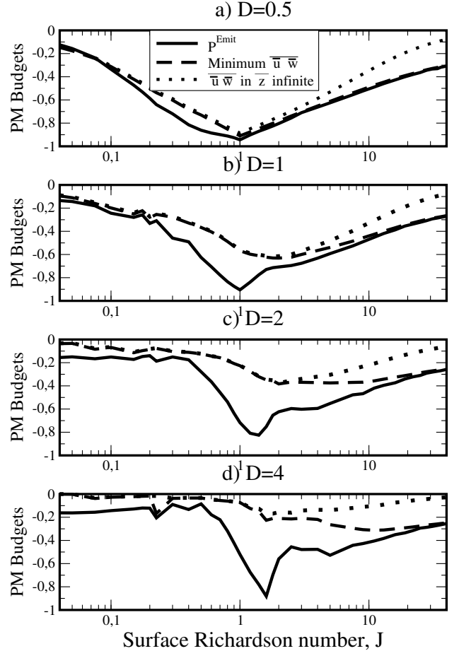
FIG. 9. Emitted pseudo momentum, minimum and emitted value of the Reynolds stress. In all simulations S = 0.15 .
