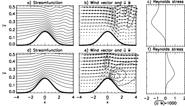
Fig. 5. Stream function (a,d), total wind vector and contours of \overline{u\bar{w}} (negative values are dashed) (b,e) and profiles of horizontally averaged Reynolds stress \overline{u\bar{w}} , S = 0.175 , D = 4 . Top panels correspond to J = 9 , bottom panels to J = 0.1 .
