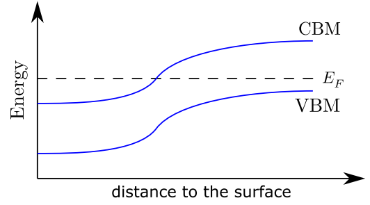
Figure 4: Schematic picture of the band bending near the surface of Bi 2 Te 3 .
