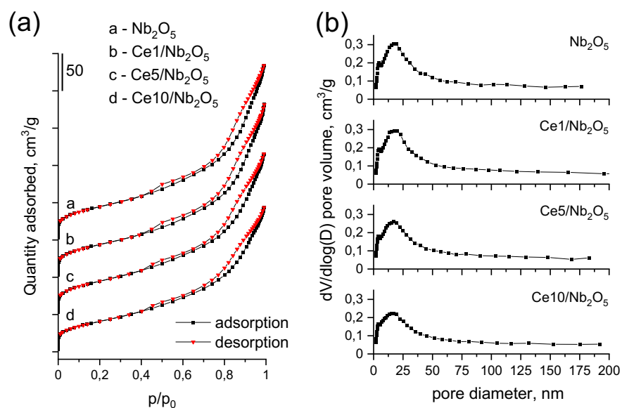
Fig. 7. (a) Low-temperature nitrogen adsorption-desorption isotherms of catalysts; (b) pore size distribution estimated for the catalysts from adsorption branch of N 2 isotherms using BJH method.
