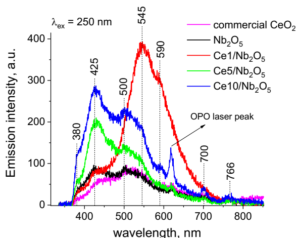
Fig. 10. Photoluminescence spectra of catalysts.
