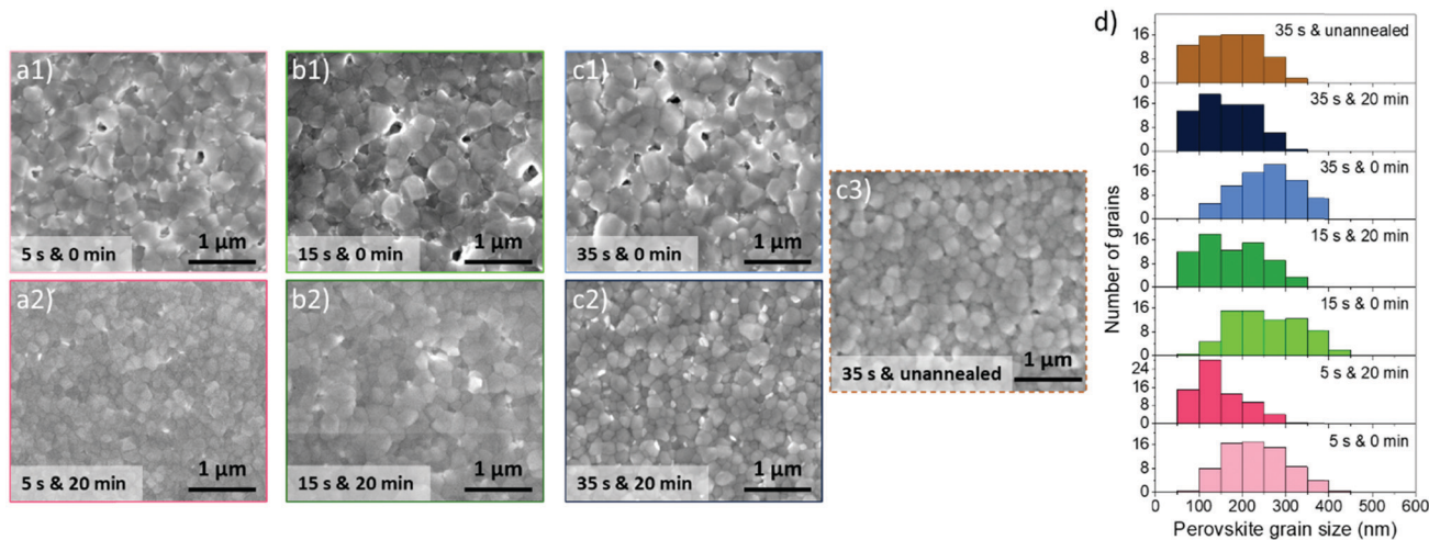
Fig. 6 (a)–(c) SEM observations of perovskite layers (performed with a perovskite concentration of 1.15 \text{ mol L}^{-1} ) for different “ t_{\text{ASE}} \& t_{\text{DBA}} ”; and (d) corresponding grain size distributions.
