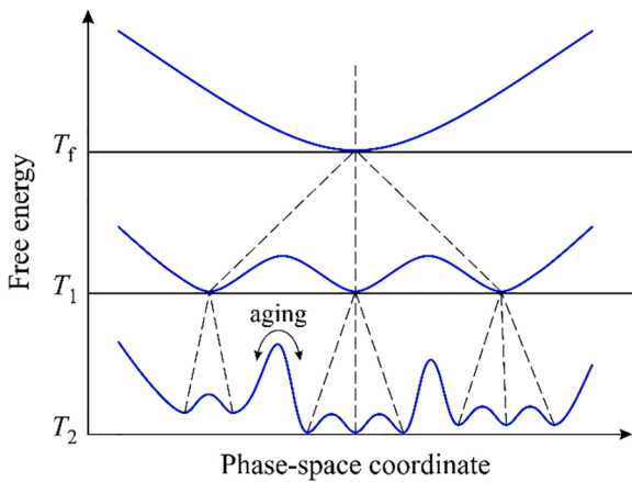
Fig. 13. Free-energy surface for the ultrametric organization of metastable states in spin glasses [27,29]. When the temperature is lowered ( T_2 < T_1 < T_f ), each valley subdivides into others. The barriers between valleys “born” from the same ancestor state are small, whereas they are increasingly higher for states that have the closest common ancestor higher on the hierarchical tree (shown by the dashed lines). Aging denotes jumping of the system over potential barriers during the waiting (aging) time t_w .
