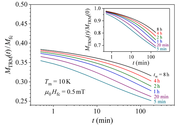
Fig. 9. TRM time-decay curves, normalized to the magnetization prior to cutting the field to zero, M_{TRM}(t_w, t)/M_{fc}(t_w) at T_m = 10 \text{ K} , as a function of the aging time t_w . The inset shows the TRM decay curves normalized to their t = 0 values, M_{TRM}(t_w, t)/M_{TRM}(t_w, t=0) , as a function of t_w .
