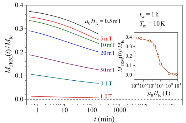
Fig. 10. TRM time-decay curves, normalized to the magnetization prior to cutting the field to zero, M_{TRM}(H_{fc}, t)/M_{fc}(H_{fc}) , at T_m = 10 \text{ K} , as a function of the aging field H_{fc} . The inset shows the TRM t = 0 amplitude, M_{TRM}(H_{fc}, t=0)/M_{fc}(H_{fc}) , as a function of H_{fc} (note that the H_{fc} scale is logarithmic).
