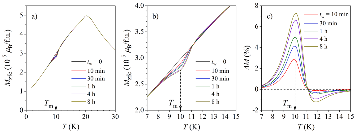
Fig. 11. (a) M_{zfc} curves obtained for different aging times t_w = 10 \text{ min}, 30 \text{ min}, 1 \text{ h}, 4 \text{ h} and 8 \text{ h} at T_m = 10 \text{ K} . (b) Expanded portions of the M_{zfc} curves in the vicinity of T_m . (c) normalized difference between the reference (unaged) curve M_{zfc}(t_w = 0) and the aged curves, \Delta M = [M_{zfc}(t_w = 0) - M_{zfc}(t_w)]/M_{zfc}(t_w = 0) .
