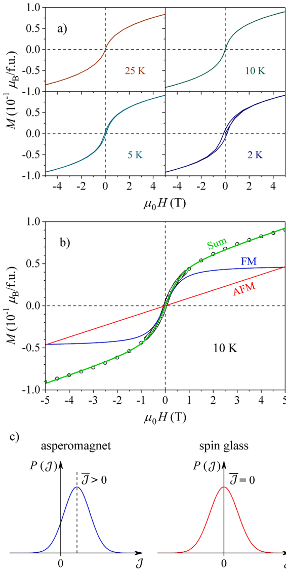
Fig. 7. (a) The magnetization versus the magnetic field curves, M(H) , at selected temperatures between 25 and 2 K. (b) The fit of the M(H) curve at T = 10 \text{ K} with Eq. (1) (fit parameters are given in the text), where the FM and AFM contributions to the total M are also shown separately. (c) Schematic presentation of the distribution function of the exchange coupling constants P(J) for a spin glass ( \bar{J} = 0 ) and asperomagnet ( \bar{J} > 0 ).
