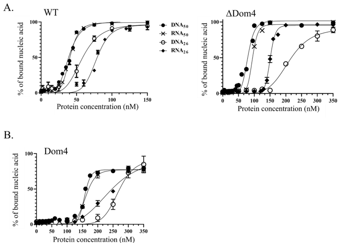
Figure 6. Binding affinities of wild type (WT) Tbar -aLhr2 and derivatives for single-stranded nucleic acids. (A) Using WT and \Delta Dom4 Tbar -aLhr2, the percentage of nucleoprotein complex formed after 15 min of incubation was plotted against the protein concentrations. The experiments were carried with RNA 50 , RNA 26 , DNA 50 and DNA 26 substrates (Supplementary Table S4). Three independent experiments were performed in each condition. (B) Identical assays were performed with a recombinant protein corresponding to Domain 4 alone.
