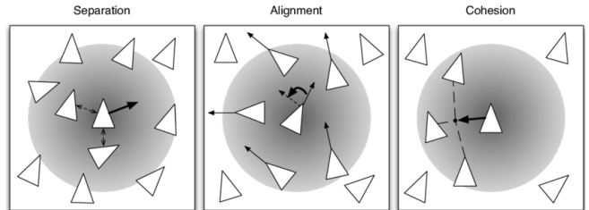
Fig. 1: Flocking : The 3 interactions defined by Reynolds (illustration from [8])
