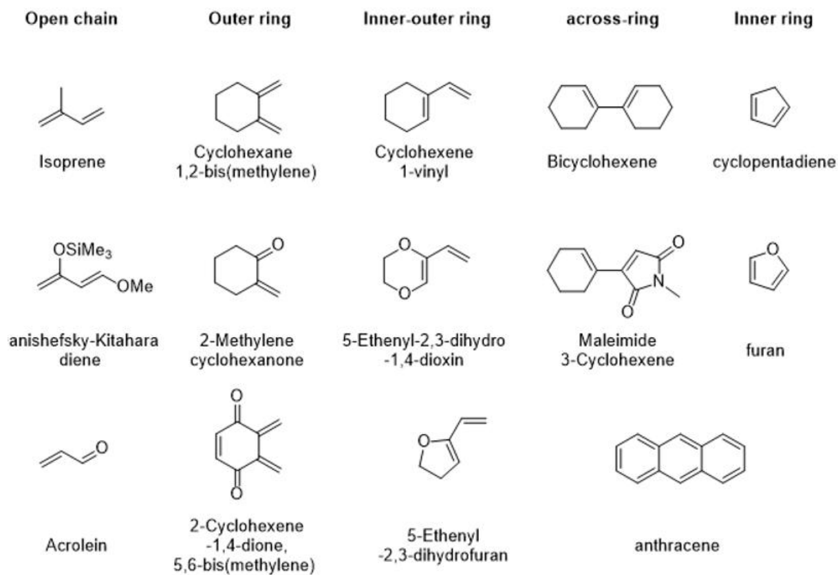
Figure 3 : List of well-known representative diene structures involved in DA reactions
