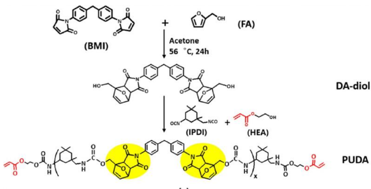
Scheme 21 : The synthetic strategy of polyurethane acrylate based on DA dynamic reversible bonding (PUDA) [145] (reproduced from ref [145] with permission from Elsevier, copyright 2020)]
