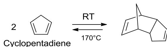
Scheme 22 : Dimerization of cyclopentadiene [173]
