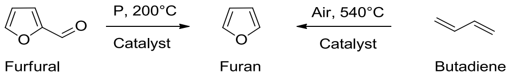
Scheme 3 : Industrial pathways from furfural or butadiene to produce furan [52, 53] [54]
