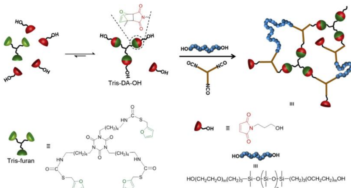
Figure 13 : Schematic representation of a thermoreversible network based on polydimethylsiloxane [154].
