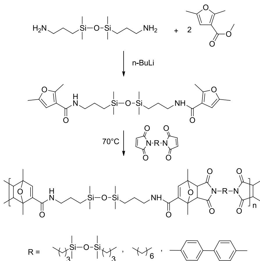
Scheme 10 : Functionalization and DA polyaddition containing siloxane moieties [90]
