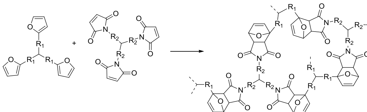
Scheme 14: Example of a crosslinked F/M network pathway
