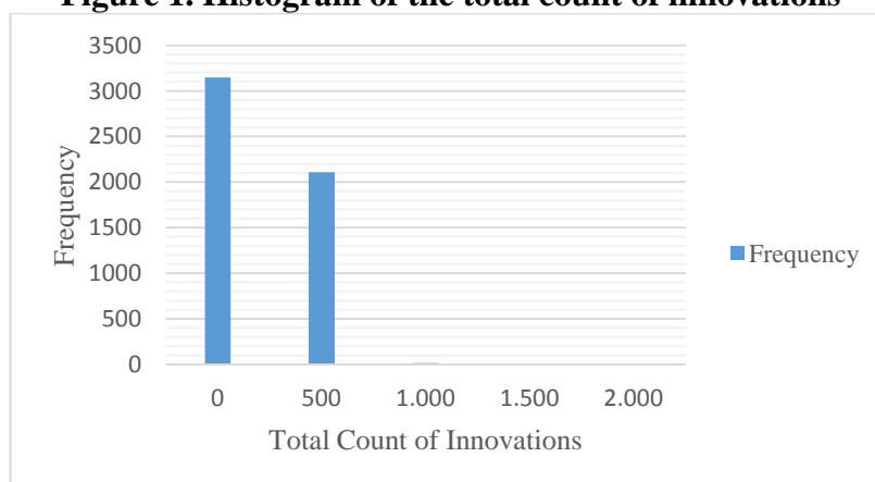
Figure 1. Histogram of the total count of innovations
