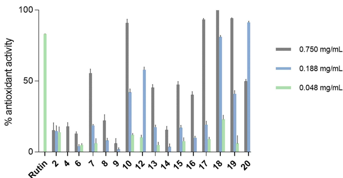
Figure 3. Antioxidant activity (%) is measured using DPPH assay at 48 \mu g/ml (green), 188
