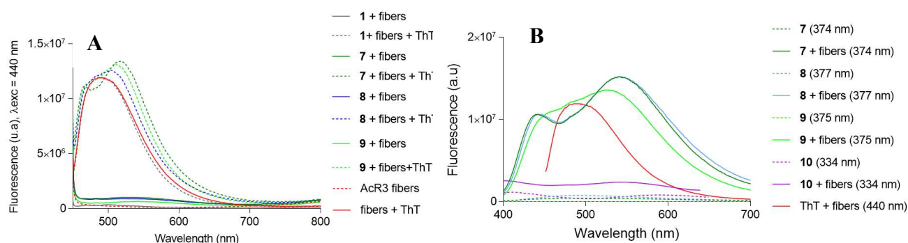
Figure 7. (A) ThT displacement assay. The excitation wavelength is 440 nm. The ratio compound/ThT is 10/1 (100/10 μM) and the AcR3 fibers have been prepared from 100 μM of peptide in presence of ThT. (B) Fluorescence emission of Ind-PyC2 compounds (100 μM) alone and in presence of 100 μM of pre-formed fibrils. The excitation wavelength corresponds to their absorbance maximum (value in parentheses); ThT in presence of fibers is used for comparison.
