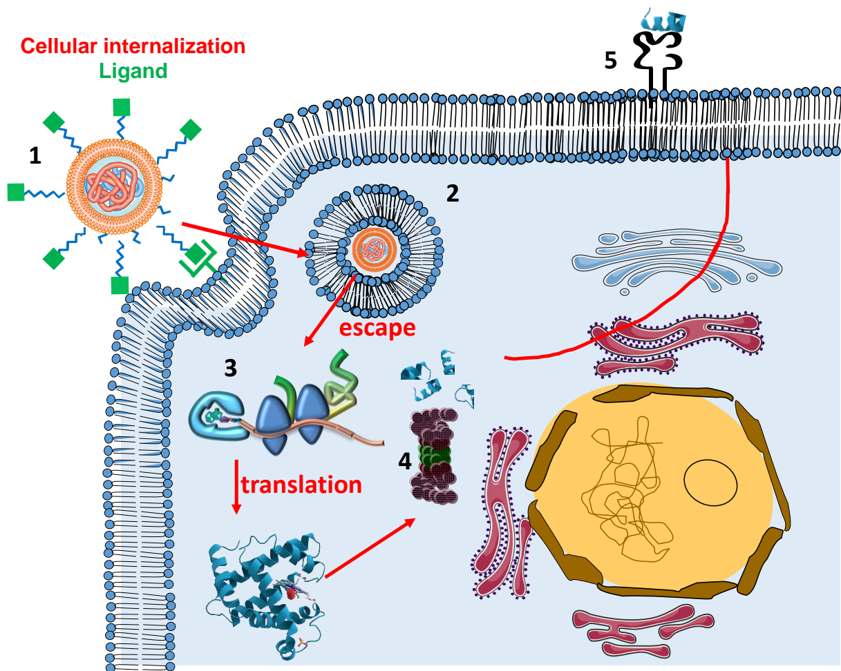
Figure 2: Critical steps in mRNA vaccine delivery: 1-recognition of targeted formulation by the cognate receptor in DC; 2- confinement of mRNA formulation inside endosome; 3-mRNA recruitment to the ribosome; 4-proteasome degradation of antigen; 5-antigenic presentation via major histocompatibility class I (MHC I) as an example).
