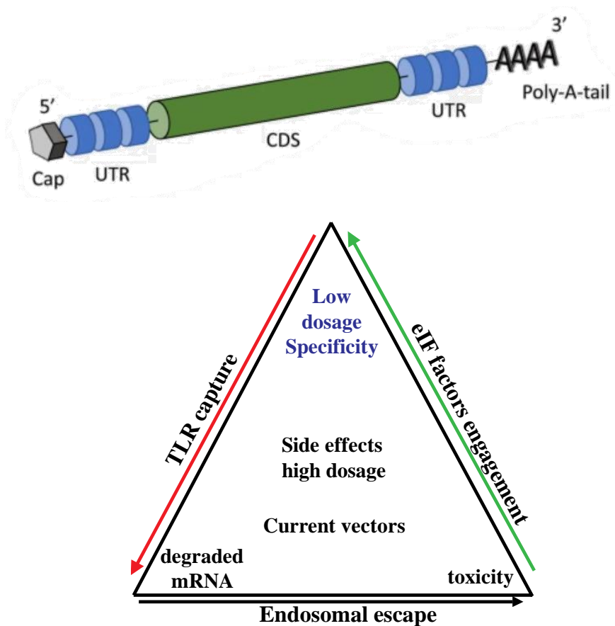
Figure 1: Schematic IVT mRNA structure and intracellular recognition of mRNA
