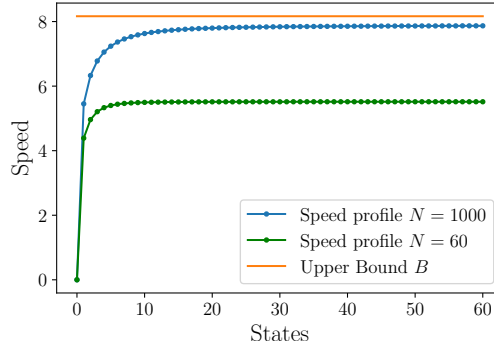
Figure 3: Two optimal speed policies in \mathcal{M}_N , for N = 60 and N = 1000 and the bound B = \sqrt{\frac{C}{3}} .
