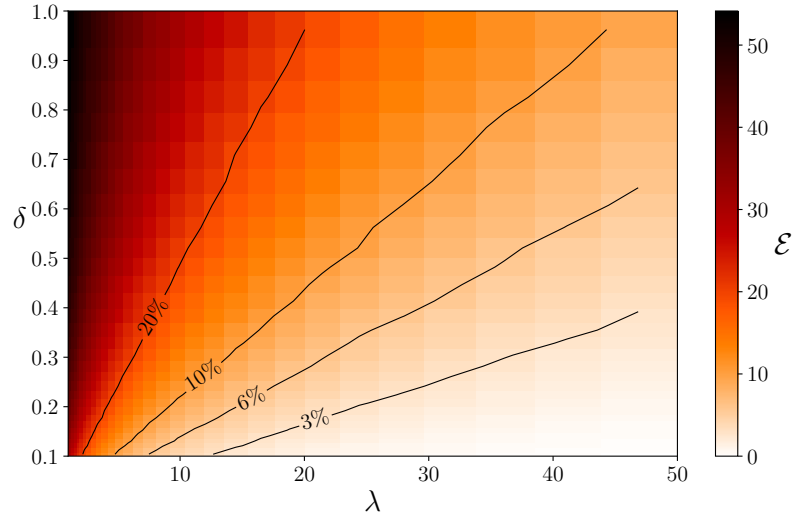
Figure 5: Level sets of the percentage relative error \mathcal{E} with a fixed miss probability p_M = 0.1 . The darker (lighter) the zone, the higher (lower) the error.
