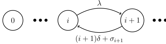
Figure 1: Markov chain diagram under policy \sigma .
