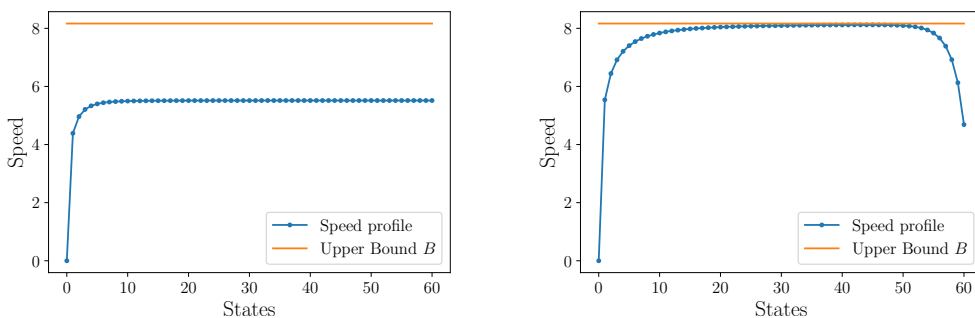
(a) \mathcal{M}_N with decaying arrival rates (b) \mathcal{M}'_N with no decay of the arrival rates
