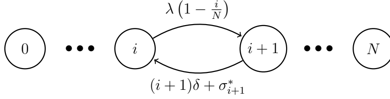
Figure 4: The transition rates of the Markov chain X^* .
