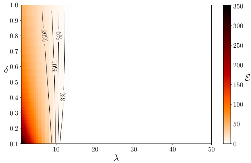
Figure 6: Level sets of the percentage relative error \mathcal{E} with a fixed cost per deadline, C = 300 .
