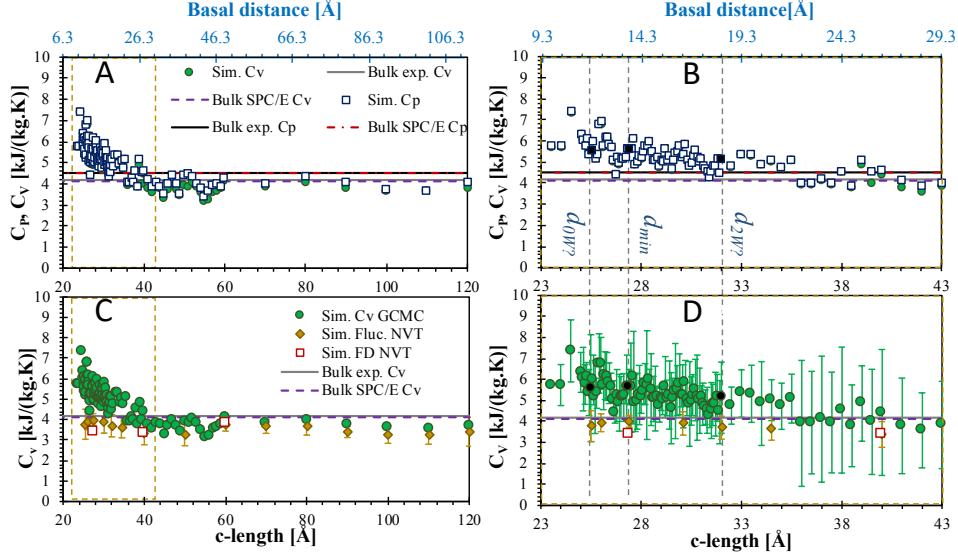
Figure 12: Heat capacity at constant volume C_V and at constant pressure C_P as a function of the c-length. In (A) the entire range of c-length is displayed; in (B), we zoom in the 23-40 Å range to highlight the values associated with the basal spacings d_{0W?} , d_{min} and d_{2W?} . The experimental and SPC/E model values of the heat capacities are taken from refs. [72] and [73], respectively. (C) Comparison of C_V of confined water computed using GCMC simulations, and NVT simulations in finite difference (FD, Eq. 24) and fluctuation (Eq. 25) approaches. In (D), we zoom in the 23-40 Å range to highlight the values associated with the basal spacings d_{0W?} , d_{min} and d_{2W?} . The standard deviations are shown for GCMC results only in (D) for the sake of readability.
