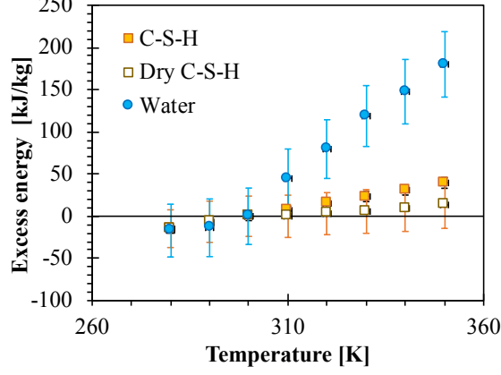
Figure 13: Excess energy with respect to the energy at T = 300 K for water saturated C-S-H (system at equilibrium basal spacing d_{min} ) obtained in NVT simulations. The energy was computed for the whole system (C-S-H), water, and "dry" C-S-H (i.e only the particles in the solid layers and interlayer ions).
