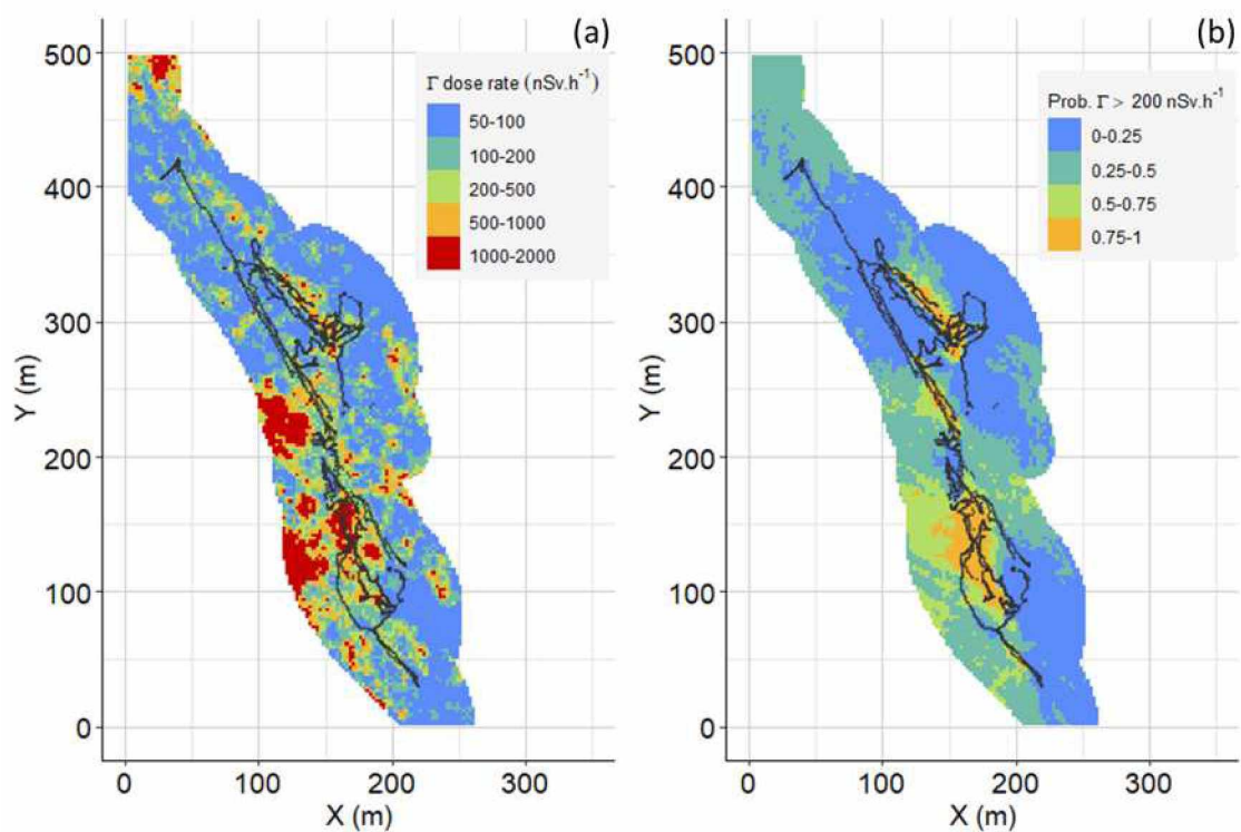
Fig. 5. One realization of a gamma dose rate field simulated by kriging of the measured values (a); and the probability of exceeding a gamma dose rate value of 200 \text{ nSv}\cdot\text{h}^{-1} , i.e., two times the geochemical background mean value (often considered to identify anthropic signal), computed based on 100 realizations (b). The black dots correspond to the location of the measurements.
