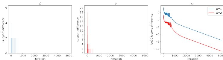
FIG. 1. Support change for the first (a) and the second (b) factor in PALM. The norm of the difference between two consecutive factors updates is depicted in (c) (logarithmic scale).
