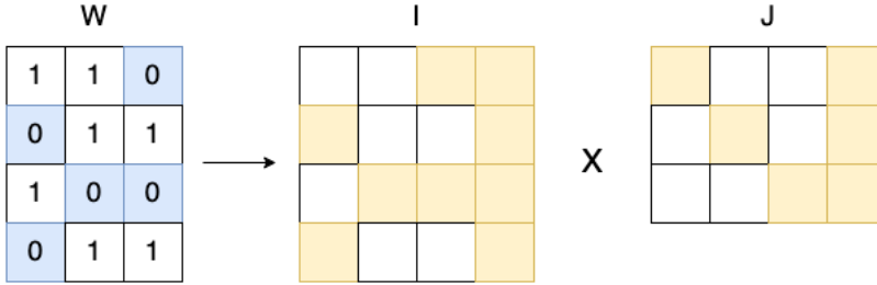
FIG. 12. Factor supports I and J constructed from the weighted matrix W \in \{0, 1\}^{4 \times 3} . Colored squares in I and J are positions in the supports.
