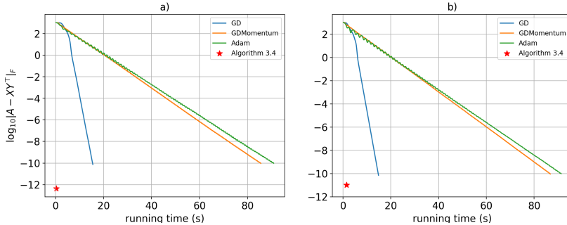
FIG. 10. Evolution of \log_{10} \|A - XY^T\|_F for three variants of gradient descent and Algorithm 3.4 with support constraints (I_1, J_1) (left) and (I_2, J_2) (right) for N = 10 .
