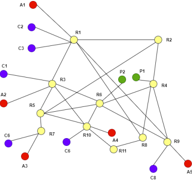
Fig. 2. DFN topology
