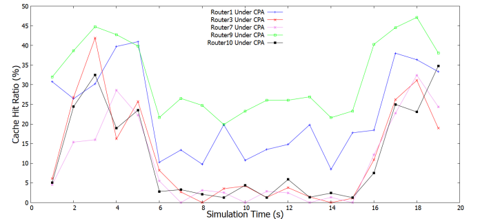
Fig. 5. Cache Hit Ratio of each edge router per time of simulation in the DFN topology
