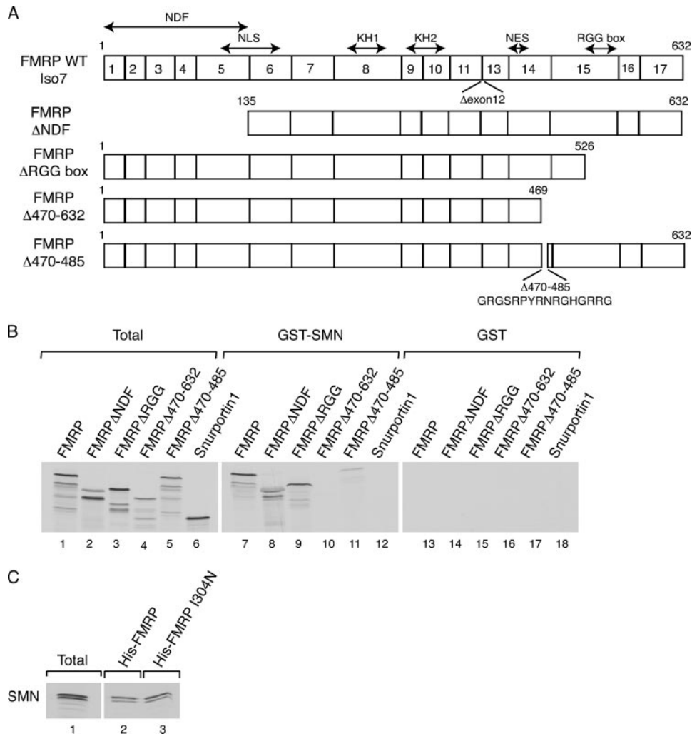
FIGURE 5. A small COOH-terminal region of FMRP is necessary for interaction with SMN. A , schematic representation of FMRP wild-type and deletion mutants used in binding assays. Regions denoted 1–17 correspond to the regions encoded by exons 1–17. Wild-type FMRP Iso7 has been used. It lacks the region encoded by exon 12 and is the most frequent FMRP isoform (150). NDF (NH 2 -terminal domain of FMRP), NLS (nuclear localization signal), NES (nuclear export signal), KH1 , KH2 , and the RGG box are indicated. The sequence spanning amino acids 470–485 is shown. B , in vitro translated [ 35 S]methionine-labeled wild-type FMRP or the indicated deletion mutants were incubated either with recombinant GST-SMN immobilized on beads (lanes 7–12), or with GST alone used as a negative control (lanes 13–18). Following extensive washes, the bound proteins were analyzed by SDS-PAGE and autoradiography. The Total lanes show 10% of the labeled proteins used in each binding reaction (lanes 1–6). C , in vitro translated [ 35 S]methionine-labeled wild-type SMN was incubated with either recombinant His-FMRP (lane 2) or His-FMRP I304N mutant (lane 3) immobilized on beads. Following extensive washes, the bound proteins were analyzed by SDS-PAGE and autoradiography. The Total lanes show 10% of labeled SMN protein used in each binding reaction (lane 1).
