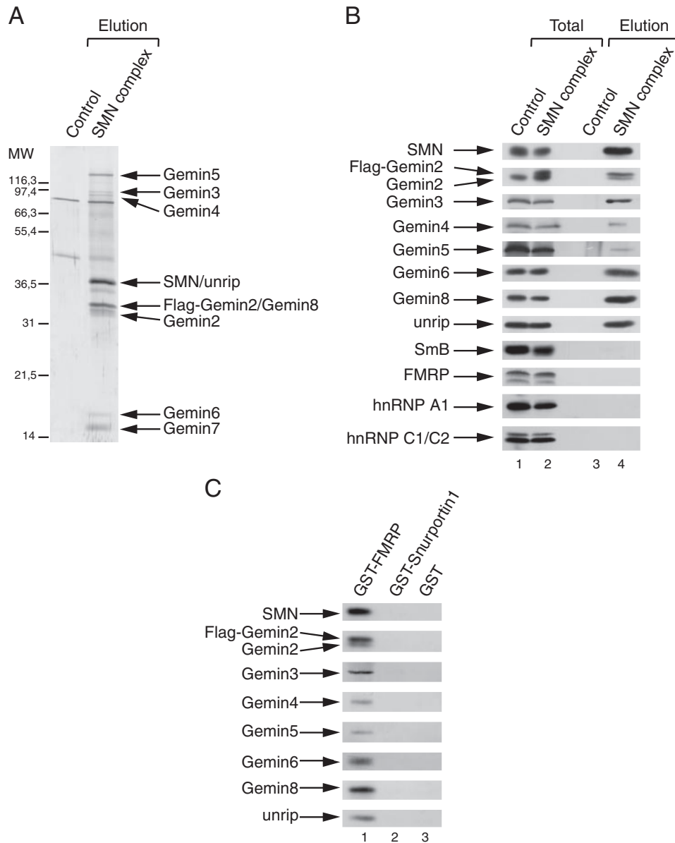
FIGURE 3. Purified native SMN complex associates with FMRP in vitro . A , native SMN complexes (SMN complex) were purified from total extracts prepared from HeLa Tet-Off cells that stably expressed FLAG-tagged Gemin2 by immunoprecipitation with anti-FLAG antibodies. After elution with an excess of FLAG peptides, the protein composition of the complexes was analyzed by SDS-PAGE followed by silver staining (Elution). The nonspecific proteins purified from HeLa Tet-off cells that do not express FLAG-Gemin2 are shown as a control (Control). The protein pattern was compared with those previously observed in Refs. 16, 18, and 21 and the proteins were assigned to known proteins of the SMN complex according to their molecular weights (MW). The identity of the proteins was confirmed by Western blotting analysis (see B ). B , the purified native SMN complex (SMN complex) shown in A was analyzed by SDS-PAGE and Western blotting with antibodies directed against the indicated proteins (Elution, lane 4). A control experiment was performed with HeLa Tet-Off cells that do not express FLAG-Gemin2 (Elution, lane 3). Lanes 1 and 2 correspond to 8% of the cellular extracts used in each assay. C , purified native SMN complexes shown in A and B were incubated with recombinant GST-FMRP immobilized on beads (lane 1), GST-Snurportin1 (lane 2), or GST alone (lane 3). The bound proteins were analyzed by SDS-PAGE and Western blotting with antibodies directed against the indicated proteins. Lane 4 of B was loaded with 25% of the amount of SMN complex used in each binding reaction.
