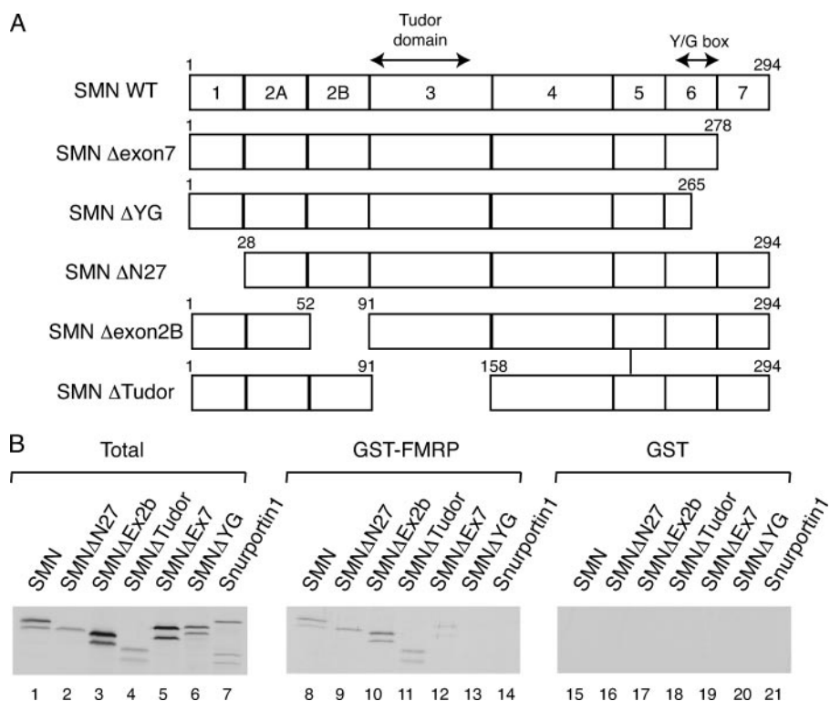
FIGURE 6. The association of SMN with FMRP requires the COOH-terminal domain of SMN. A , schematic representation of SMN wild-type and deletion mutants used in binding assays. Regions denoted 1–7 correspond to the regions encoded by exons 1–7. The Tudor domain and the YG box are indicated. B , in vitro translated [ 35 S]methionine-labeled wild-type SMN or the indicated mutants were incubated with recombinant GST-FMRP immobilized on beads (lanes 8–14), or with GST alone used as a negative control (lanes 15–21). Following extensive washes, the bound proteins were analyzed by SDS-PAGE and autoradiography. The Total lanes show 10% of labeled proteins used in each binding reaction (lanes 1–7).
