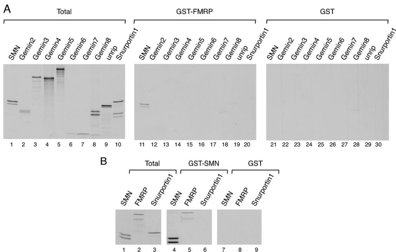
FIGURE 4. The SMN protein, but none of the other components of the SMN complex, interacts with FMRP in vitro . A , in vitro -translated [ 35 S]methionine-labeled SMN, Gemin2, Gemin3, Gemin4, Gemin5, Gemin6, Gemin7, Gemin8, Unrip, as well as Snurportin1, which was used as a negative control, were incubated with recombinant GST-FMRP immobilized on beads (lanes 11–20). Recombinant GST immobilized on beads was used as a negative control (lanes 21–30). After extensive washes, the bound proteins were analyzed by SDS-PAGE and autoradiography. The Total lanes show 10% of each labeled protein used in binding reactions (lanes 1–10). B , in vitro translated [ 35 S]methionine-labeled FMRP, as well as SMN and Snurportin1, which were used, respectively, as positive and negative controls, were incubated with recombinant GST-SMN immobilized on beads (lanes 4–6). Recombinant GST immobilized on beads was used as a negative control (lanes 7–9). Following extensive washes, the bound proteins were analyzed by SDS-PAGE and autoradiography. The Total lanes show 10% of each labeled protein used in binding reactions (lanes 1–3).
