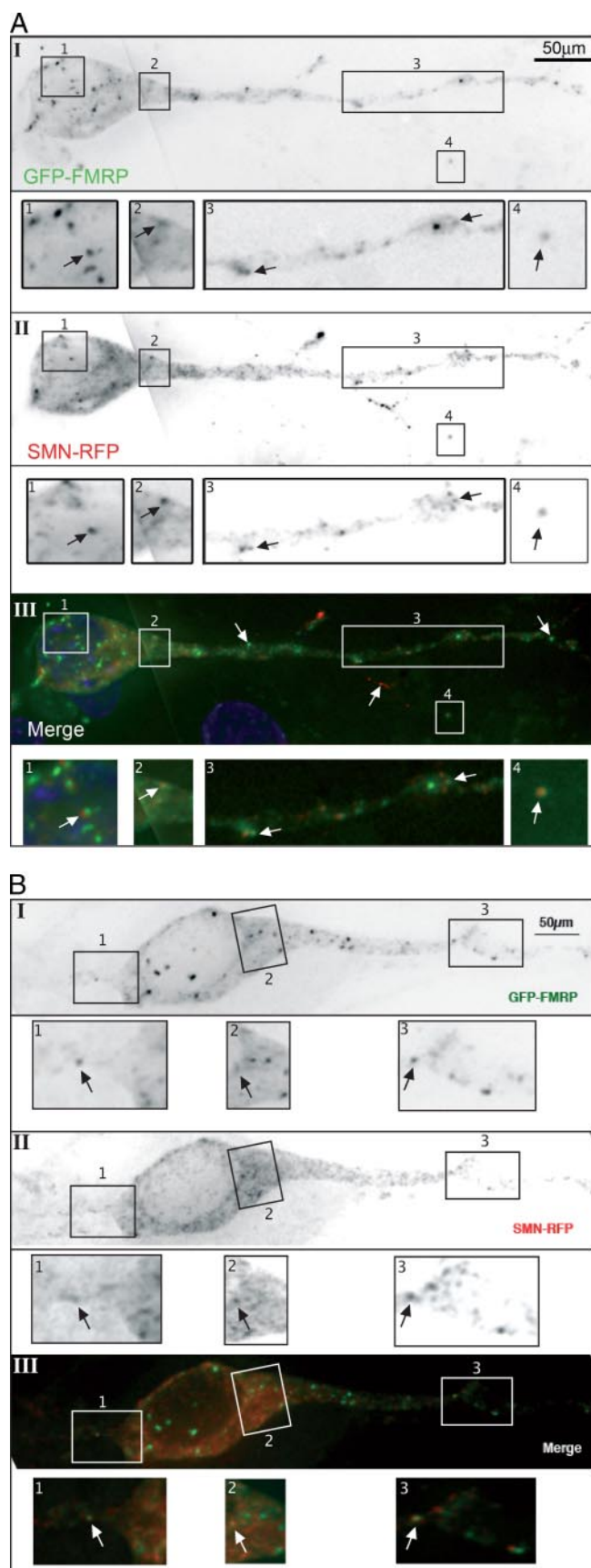
FIGURE 2. A fraction of neuronal SMN granules contains FMRP protein. A and B, rat primary neurons of hypothalamus were co-transfected with plasmids expressing GFP-FMRP and SMN-RFP fusion proteins. Localization of
