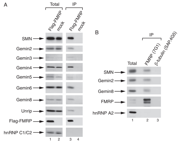
FIGURE 1. The SMN complex is associated with FMRP in human and murine neuronal cell lines in culture. A , immunoprecipitation experiments using anti-FLAG antibody (IP, lanes 3 and 4) were carried out on total extracts prepared from human neuroblastoma SH-SY5Y cells that were transiently transfected with a DNA construct expressing FLAG-tagged FMRP (Flag-FMRP, lanes 1 and 3) or the empty vector (mock, lanes 2 and 4). The immunoprecipitated proteins were analyzed by SDS-PAGE and Western blotting using antibodies directed against the indicated proteins. 2.5% of the extracts used in each experiment are shown (Total, lanes 1 and 2). B , immunoprecipitation experiments using anti-FMRP 7G1 antibody (IP, lane 2) and anti- \beta tubulin SAP.4G5 antibody (IP, lane 3) were carried out on total extracts prepared from murine motor neuron MN-1 cells. The 7G1 antibody recognizes the various FMRP isoforms. The immunoprecipitated proteins were analyzed by SDS-PAGE and Western blotting using antibodies directed against the indicated proteins. 2.5% of the extract used in the experiments is shown (Total, lane 1).
