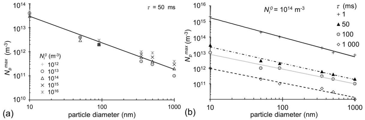
Fig. 7. Maximal aerosol concentration N_p^{max} for constant mean charge per particle within 10 % as a function of particle diameter (a) for a given charging time of \tau = 50 \text{ ms} and initial ion density N_i^0 from 10^{12} to 10^{16} \text{ m}^{-3} and (b) for a given initial ion density N_i^0 = 10^{14} \text{ m}^{-3} with charging times between 1 ms and 1 s.
