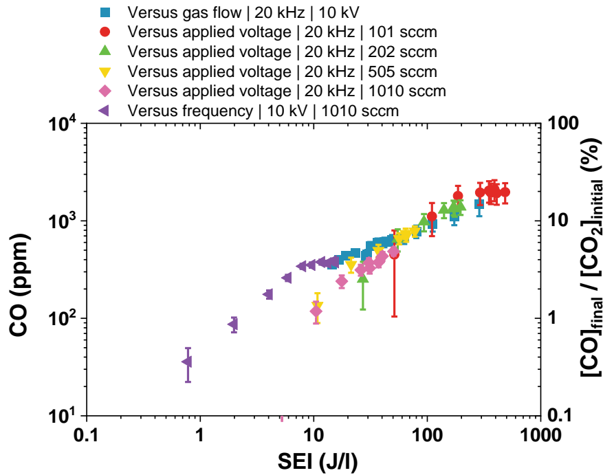
Figure 11: Conversion degree versus the specific energy input (SEI) for the all the data presented in the paper. Conditions: He with 1% CO 2 admixture.
