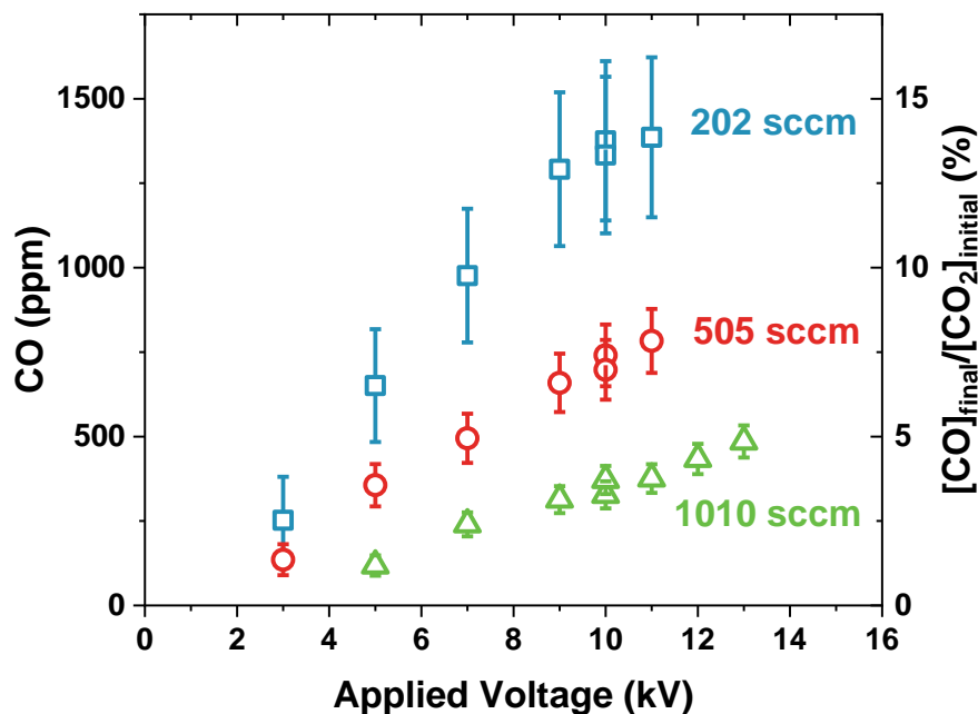
Figure 10: CO concentration versus the applied voltage at 20 kHz in He with 1% CO 2 admixture for various gas flows: 202 sccm (blue square), 505 sccm (red circle) and 1010 sccm (green triangle).
