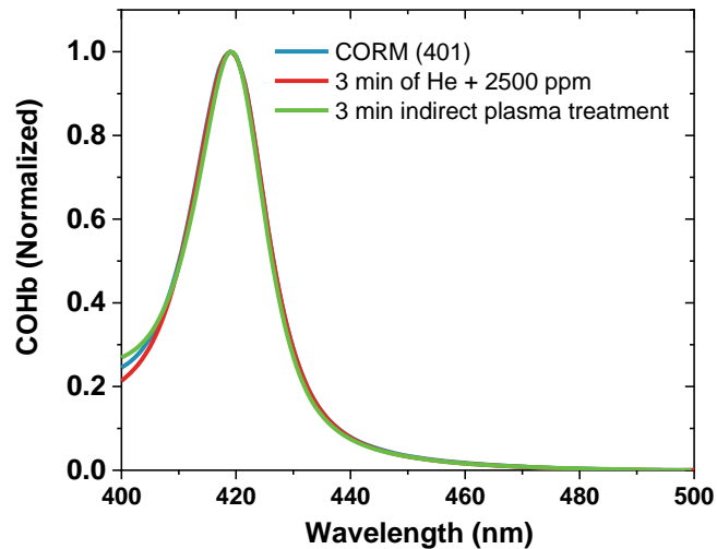
Figure 4: Comparison of the absorption spectra with 100% COHb with CORM-401 (blue), after 3 minutes of 2500 ppm CO diluted in helium gas at a flow rate of 100 sccm (red), and after 3 minutes of an indirect plasma treatment at 100 sccm of He with 1% of CO 2 at 20 kHz and 10 kV (green).
