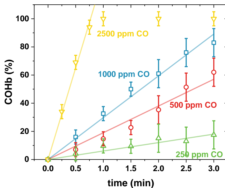
Figure 12: Percentage of COHb formation over time using various concentrations of CO diluted in helium: 250 ppm (green up-pointing triangle), 500 ppm (red circle), 1000 ppm (blue square) and 2500 ppm (yellow down-pointing triangle). Condition: 100 sccm.
