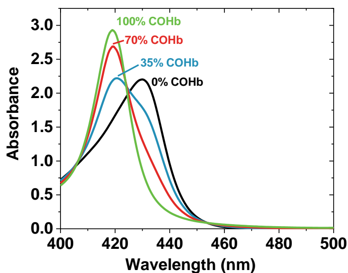
Figure 3: Absorption spectra before (black) and after the addition of 2500 ppm CO diluted in helium gas at a flow rate of 100 sccm with different treatment times (blue: 15 s, red: 30 s, green: 60 s).
