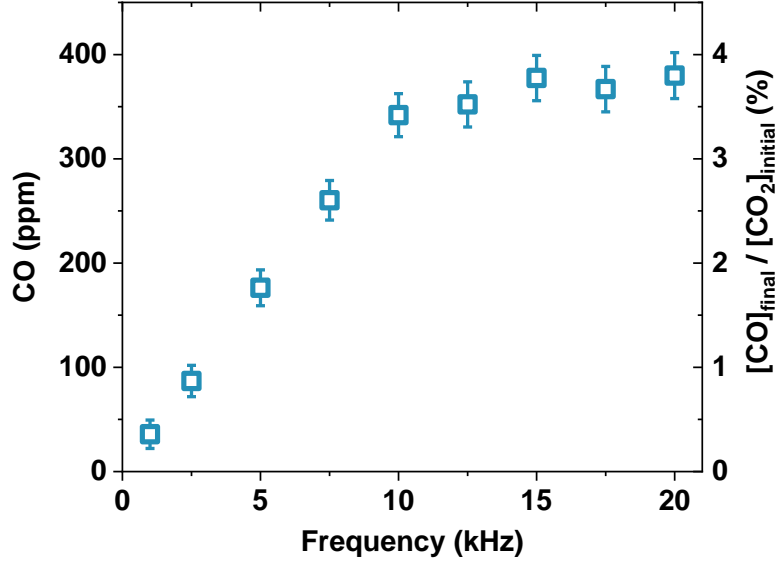
Figure 6: CO concentration versus the discharge frequency at 10 kV in helium with 1% CO 2 admixture with 1010 sccm as flow rate. The energy per cycle rose to 26.3 \pm 0.7 \mu\text{J} .
