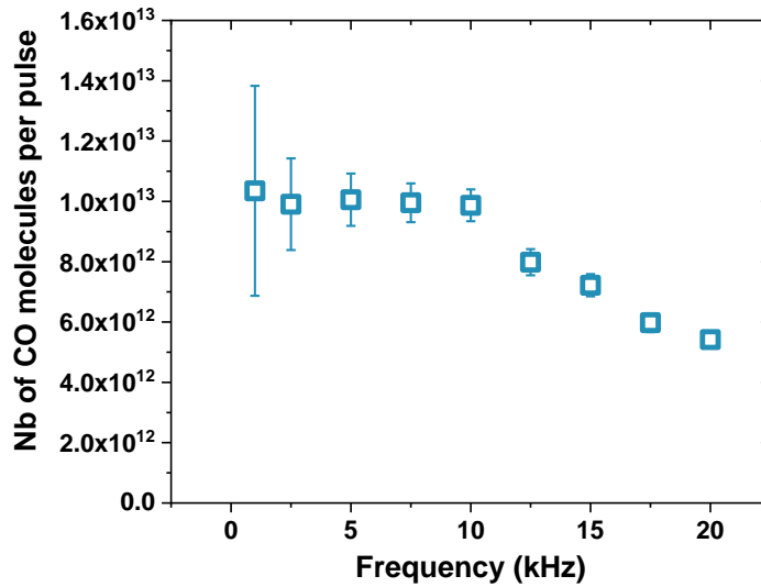
Figure 8: Number of CO molecules produced per pulse versus the frequency at 10 kV in helium with 1% CO 2 admixture with 1010 sccm as flow rate.
