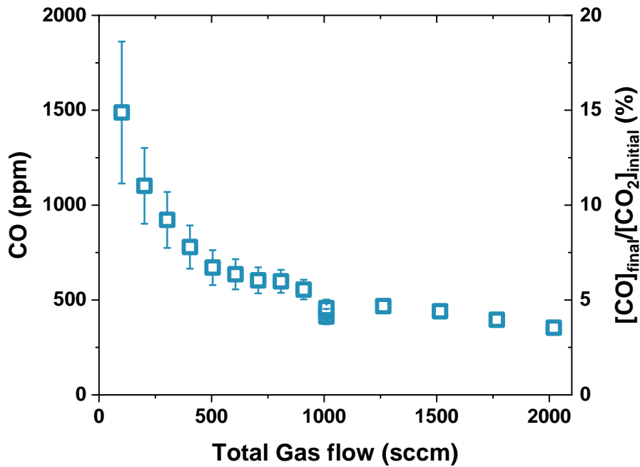
Figure 5: CO concentration (open blue square) and conversion degree versus the total flow rate in helium with 1% CO 2 admixture, with a frequency of 20kHz at 10kV.
