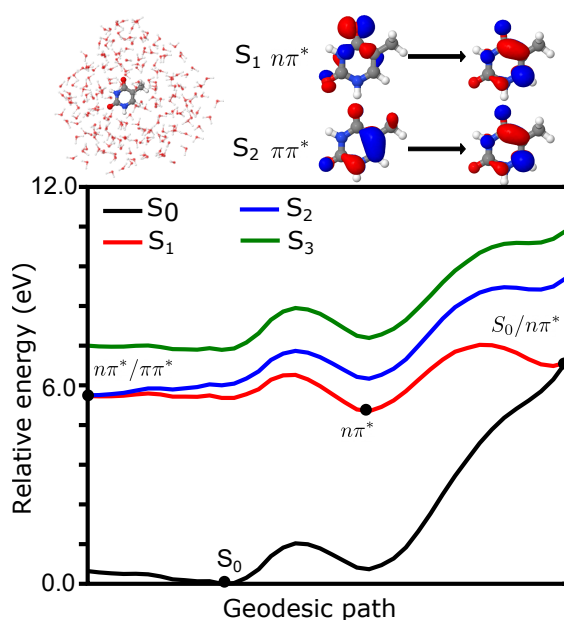
Figure 5. Photochemistry of thymine in water. ( top, left ) Schematic structure of thymine and water QM/MM model. ( top, right ) Main character of the transitions representing the first and second singlet excited states. ( bottom ) Geodesic path connecting the conical intersections between S_0/n\pi^* , S_0/\pi\pi^* and n\pi^*/\pi\pi^* as well as S_0 and n\pi^* minima. Energies (in eV) have been computed at the TDA-TDBH&HLYP/6-31G* level.
