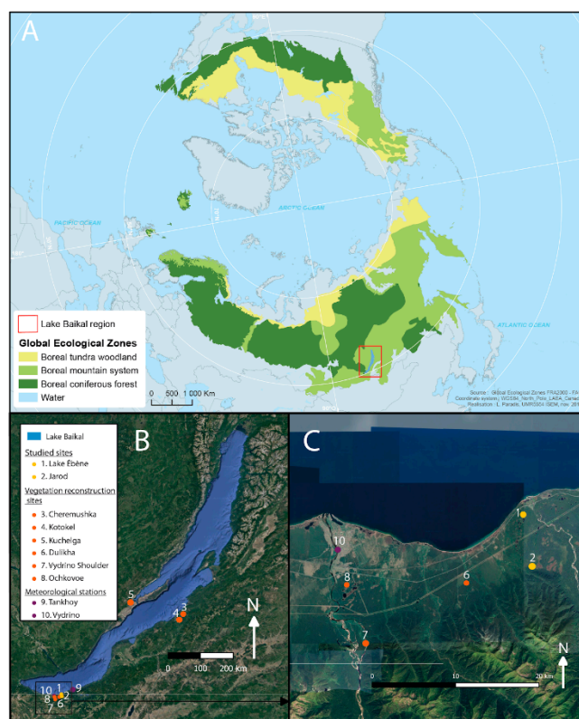
Figure 1. (A) Map of the boreal zone and location of Lake Baikal. (B) Lake Baikal and location of lakes Ebène and Jarod (1–2, this study) and available pollen records (3 to 8, orange) [36,38,46,47], and meteorological stations (pink). (C) Southern Lake Baikal region and location of Lake Ébène and Lake Jarod; Dulikha, Vydrino Shoulder and Ochkovoe pollen records; and meteorological stations.
