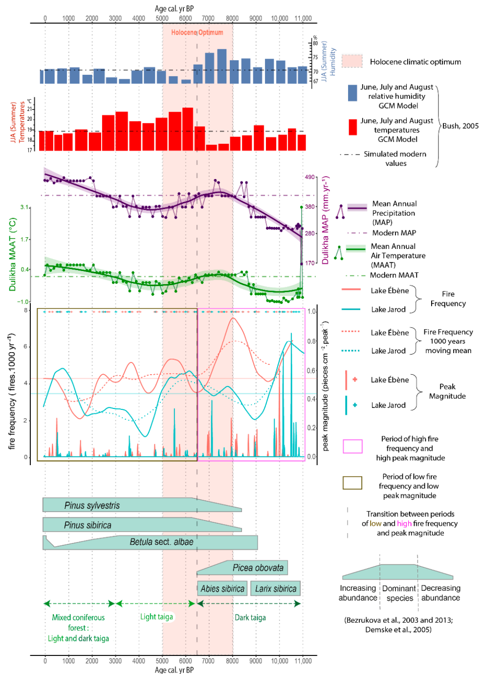
Figure 4. Correspondences in Lake Èbène and Lake Jarod fire evolutions (fire frequency, fire frequency median, fire frequency with 1000-year moving mean, fire events and peak magnitude) with summarized variations in reconstructed vegetation of the southern region of Lake Baikal during the Holocene: Vydrino (0–13,520 cal. yr BP), Dulikha (0–11,109 cal. yr BP) and Ochkovoe (0–4500 cal. yr BP) see Figure 1 [36,46,47] and reconstructed climate: temperature and precipitation for Dulikha and atmospheric general circulation model (GCM) output using a series of 500-year intervals for continental Eurasia (45–70° N, 75–130° E) that includes the Lake Baikal region [65,66].
