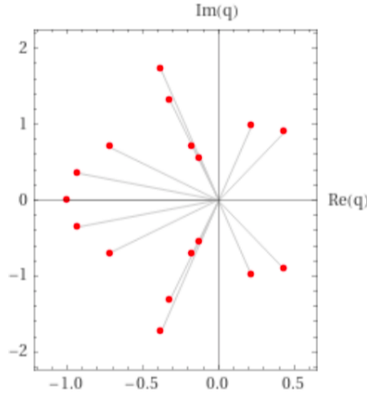
FIGURE 1. Roots of \mathcal{P}_{10}(q) : the smallest root modulus is 0.5668..., and the largest 1.8832...
