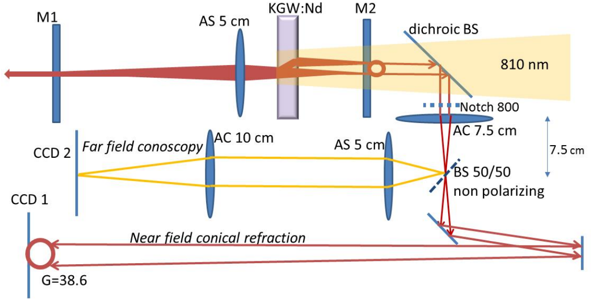
Fig. 2 Lasing set-up and optical paths for far field and near field analysis.
