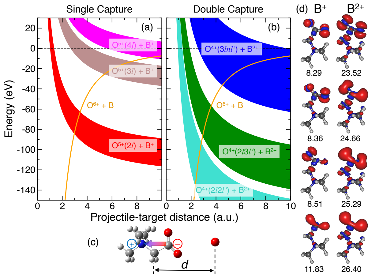
Figure 1: The O 6+ - betaine system. Molecular energies for (a) single-electron capture and (b) double-electron capture channels as a function of the distance between the O 6+ projectile and the center of mass of the betaine molecule oriented as shown in panel (c). For the sake of clarity, only the energy ranges covered by the single- and double-electron capture channels leading to O 5+ ( nl ) with n < 5 (a) and O 4+ ( 2nl' ) with n < 4 and O 4+ ( 3nl' ) (b) are shown. The missing channels are expected to be barely populated in the collision or lie outside the axes range. Notice that the incoming projectile approaches the molecule from the side of the negatively charged carboxylate group, which is the most favorable orientation for single and double capture (see text). The orange curves in (a) and (b) represent the entrance channel. The electron densities, referred to the ground state electron density of neutral betaine, for the lowest states of singly- and doubly-charged betaine resulting from single- and double-electron capture, respectively, are shown in panel (d). The numbers below the density maps indicate the energies (in eV) of the corresponding electronic states of singly- and doubly-charge betaine with respect to the energy of the ground state of neutral betaine.
