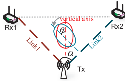
Fig. 25. Performing Gestures with different orientations
