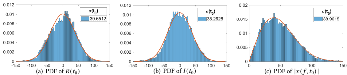
Fig. 2. Probability Distribution Function (PDF) of R(t_0) , I(t_0) and |x(f, t_0)|
