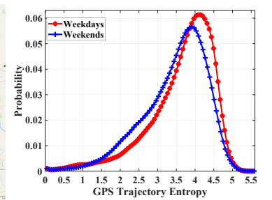
Fig. 8. The distribution of driver entropies.
