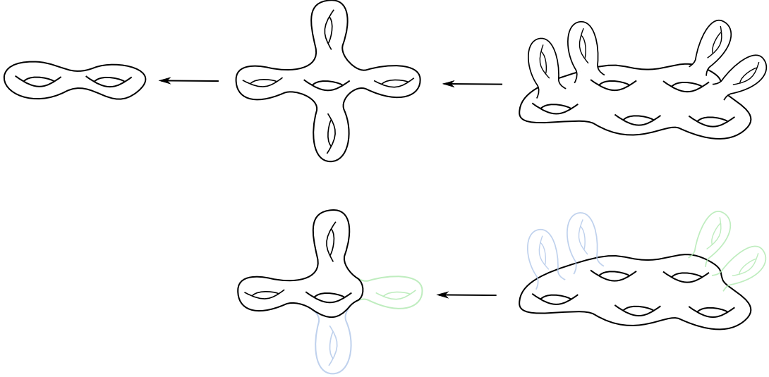
Figure 2: Illustrations of the proof of Theorem 3.4. The above line illustrates the coverings corresponding to the inclusions \Lambda \leq \Lambda_d \leq \Gamma . The bottom line illustrates the covering corresponding to the inclusion N' \leq \Lambda_d/N .
