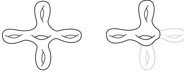
Figure 1: An illustration of the morphism that erases generators.
