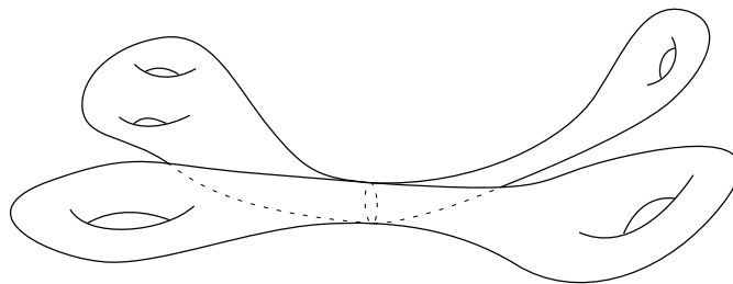
Figure 3: A branched surface
